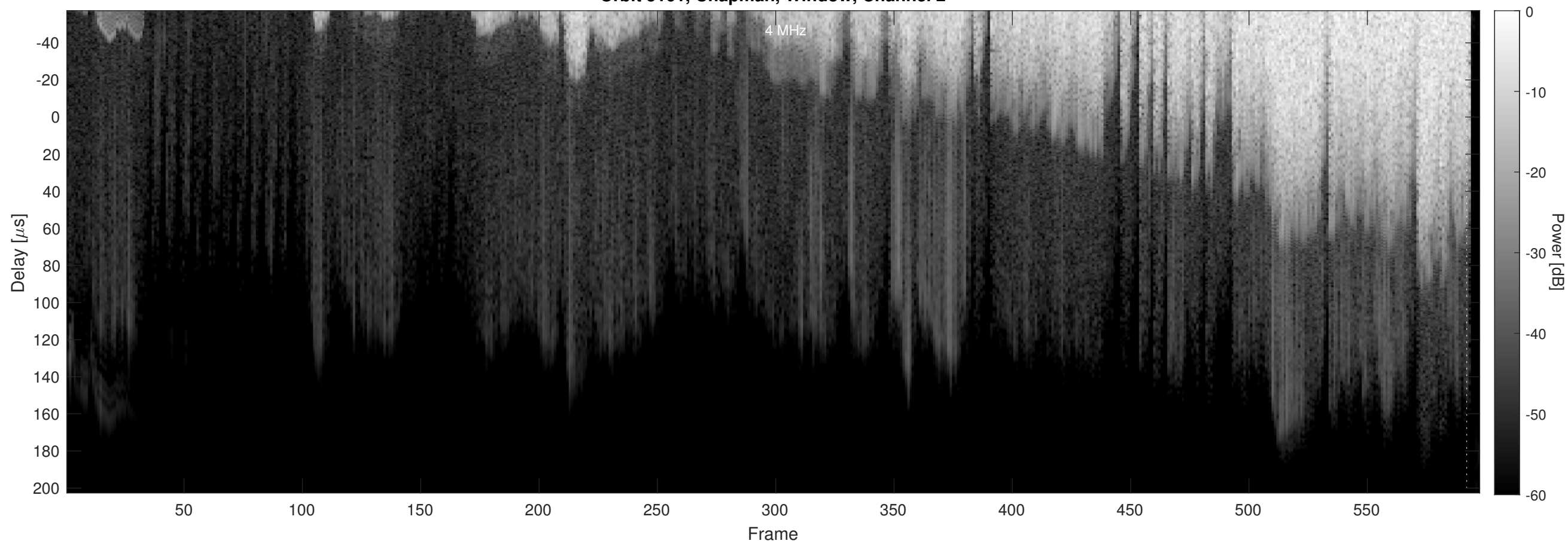
Orbit 5161, Chapman, Window, Channel 2
