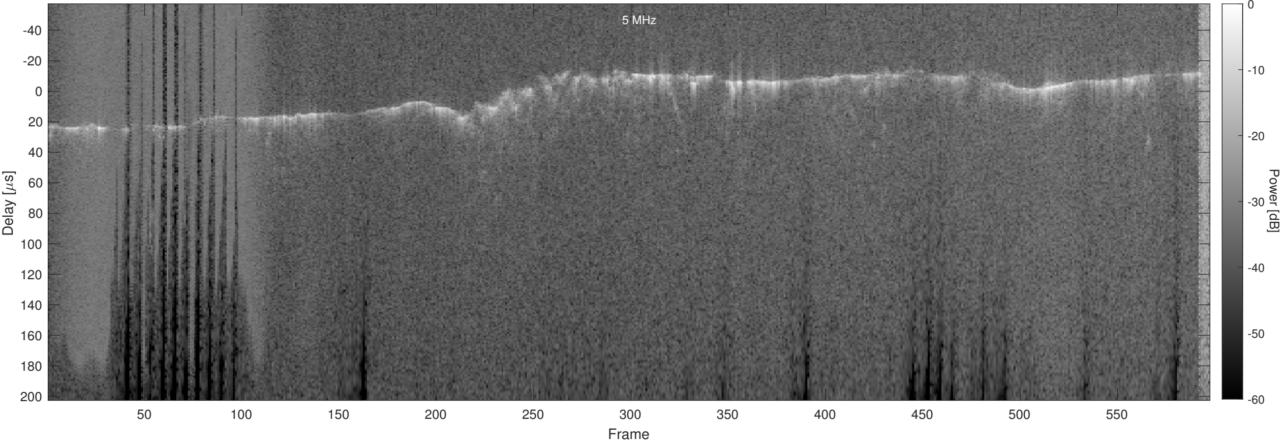
Orbit 5161, Optimized, No Window, Channel 2
