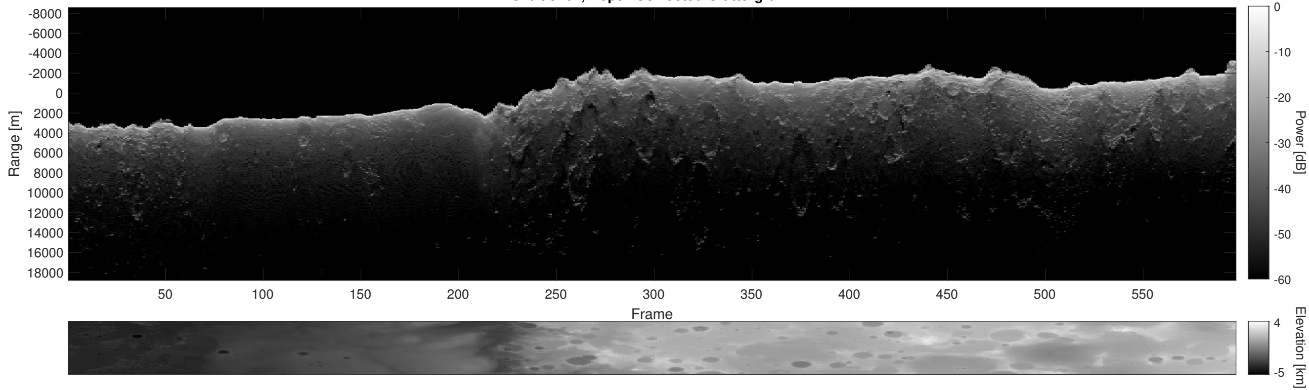
Orbit 5161, Depth-Corrected Cluttergram
