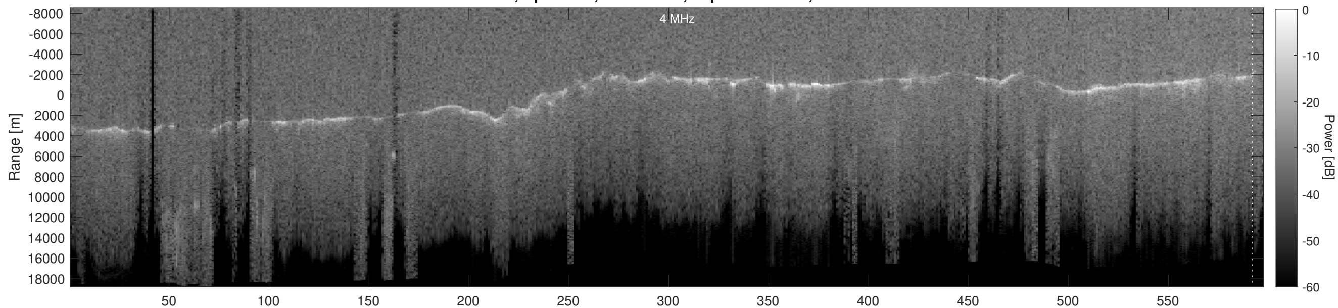
Orbit 5161, Depth-Corrected Cluttergram
