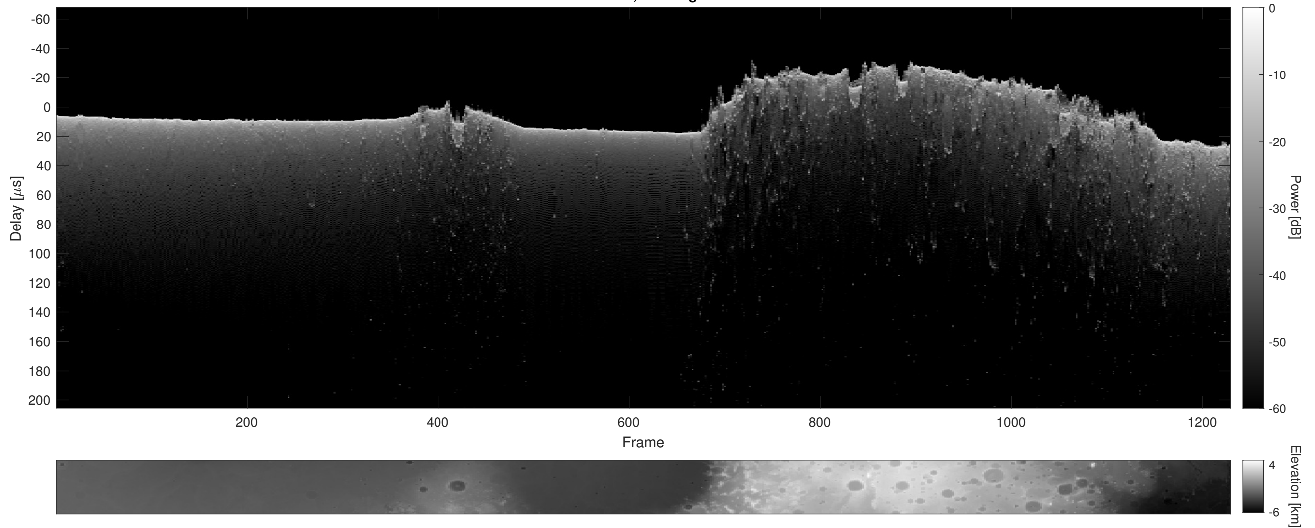
Orbit 5162, Cluttergram
