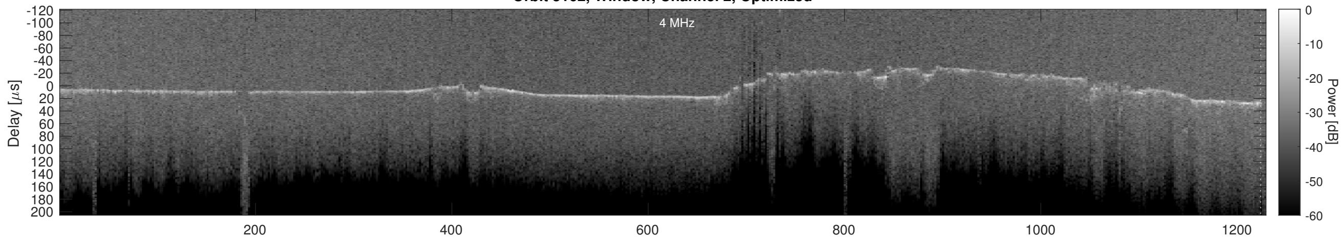
Orbit 5162, Cluttergram
