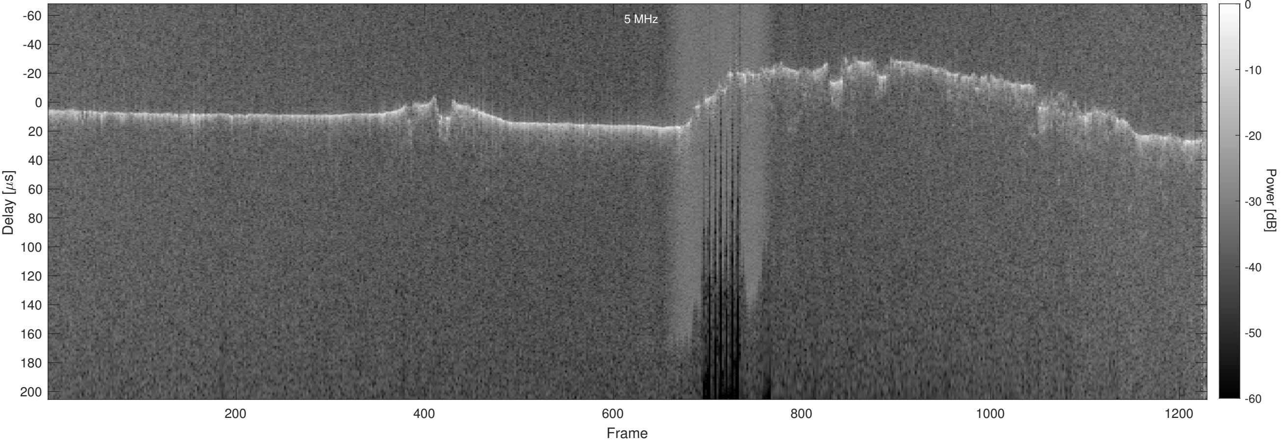
Orbit 5162, Optimized, No Window, Channel 2
