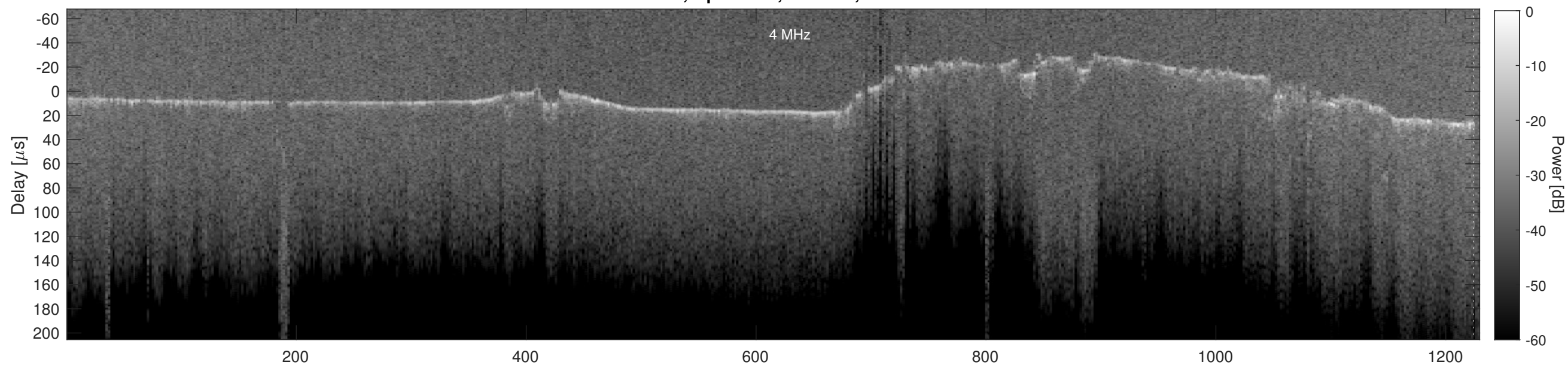
Orbit 5162, Cluttergram
