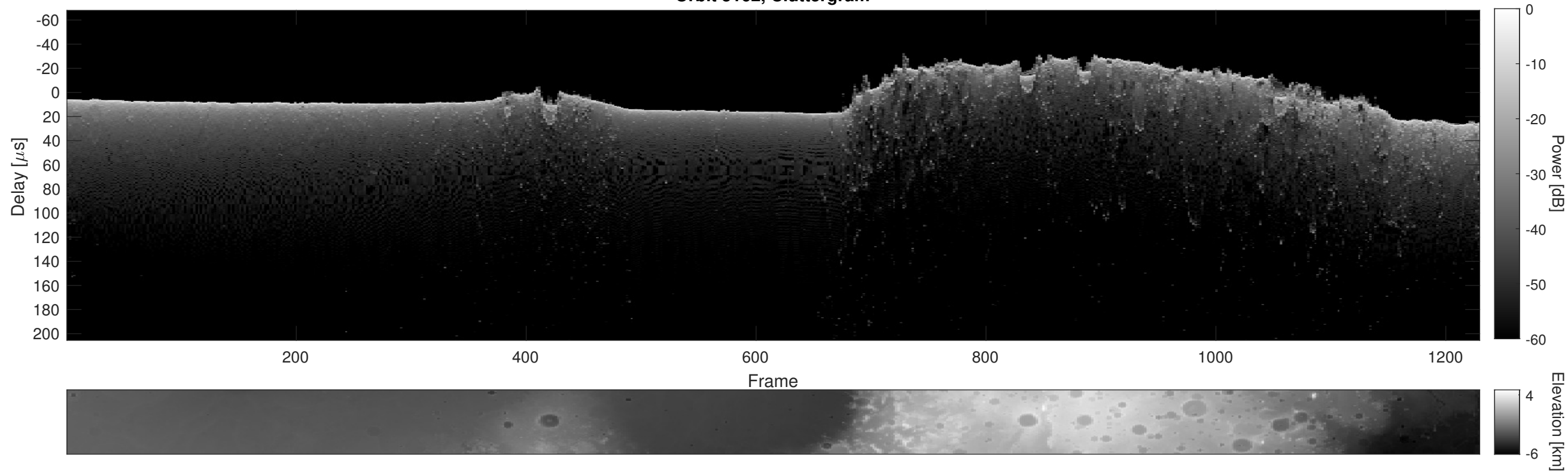
Orbit 5162, Cluttergram
