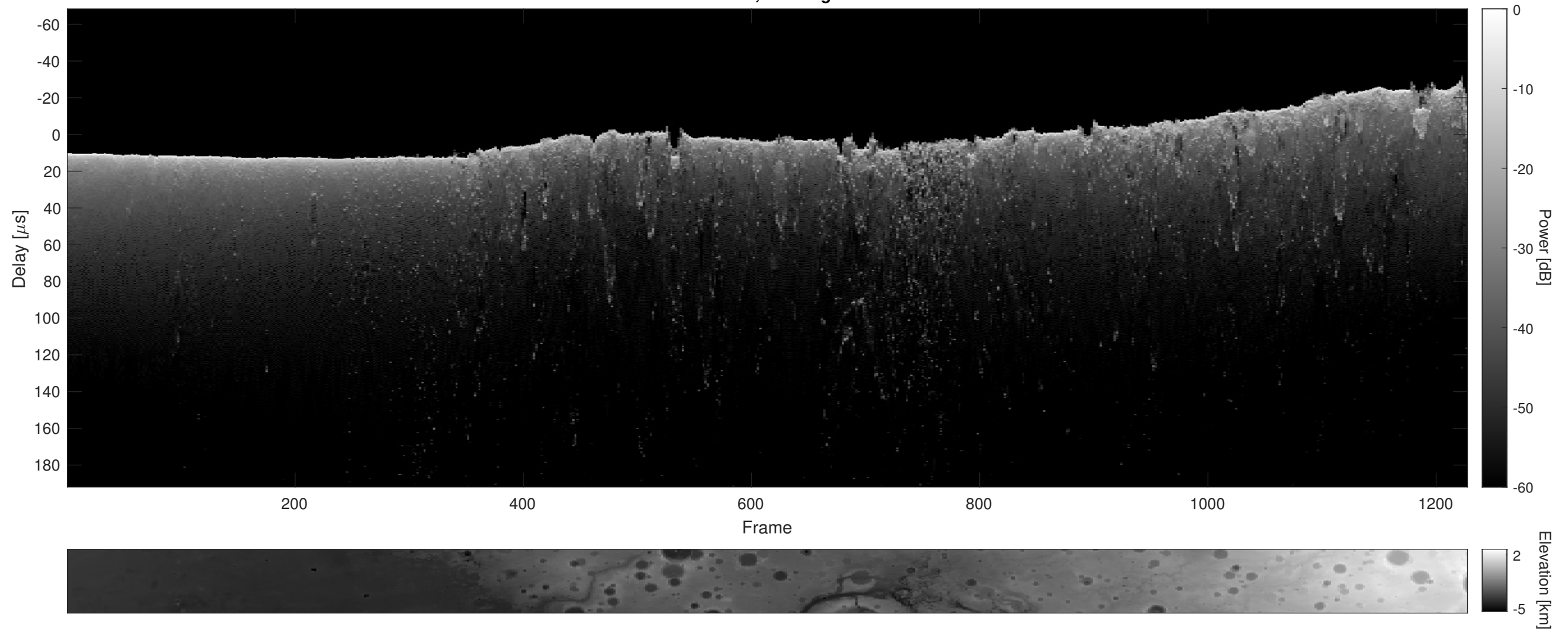
Orbit 5163, Cluttergram
