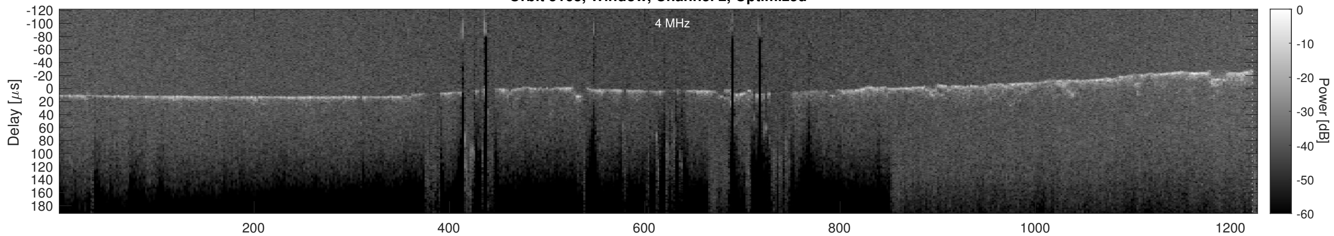
Orbit 5163, Cluttergram
