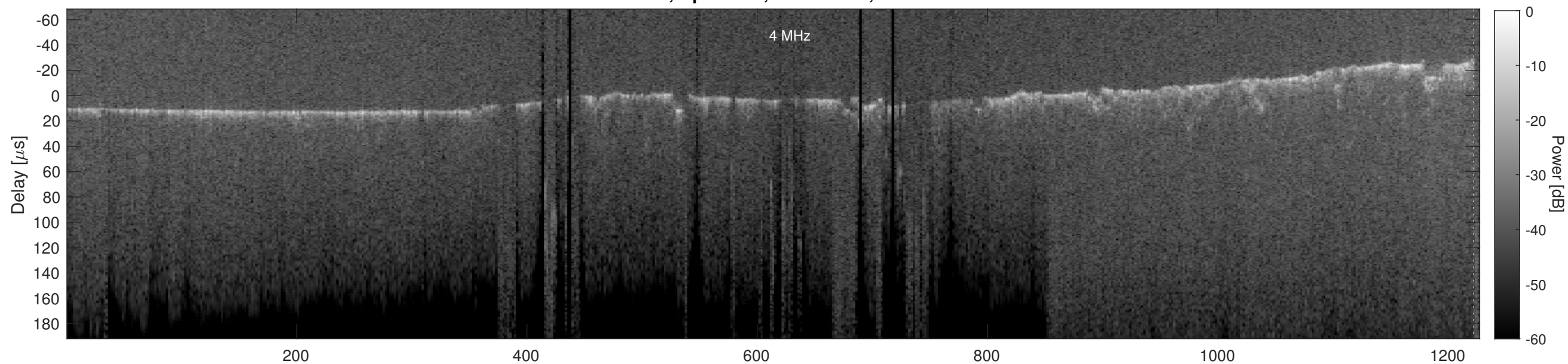
Orbit 5163, Cluttergram
