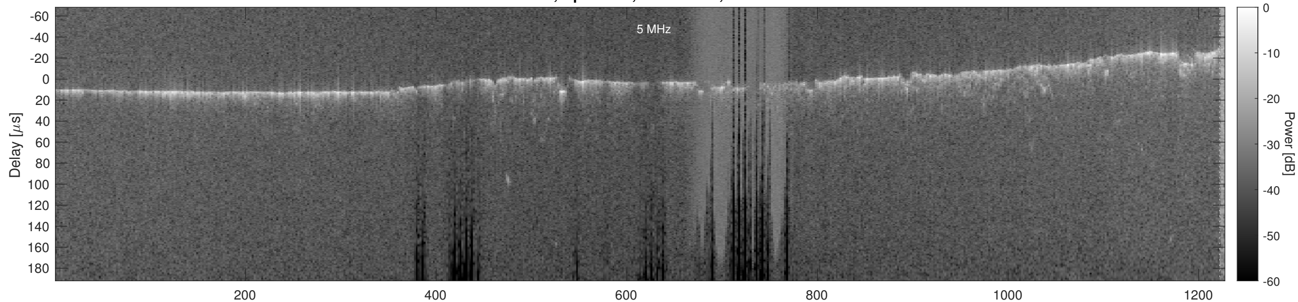
Orbit 5163, Optimized, No Window, Channel 2
