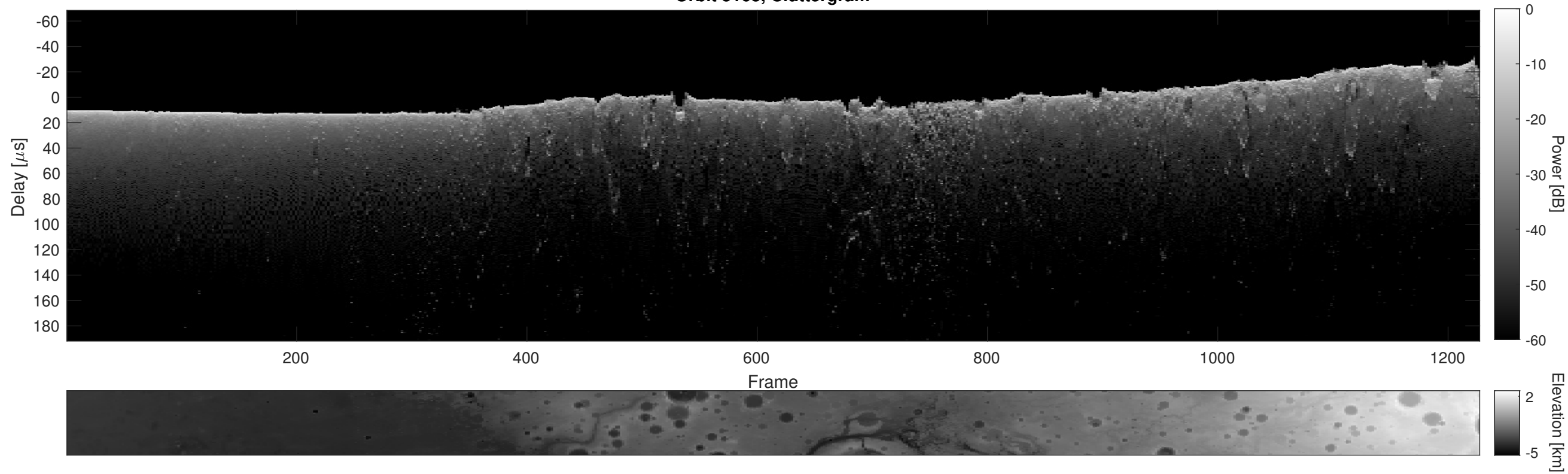
Orbit 5163, Cluttergram
