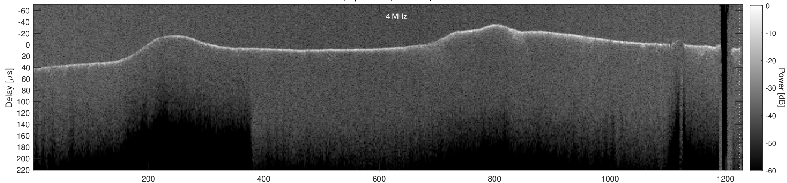
Orbit 5164, Cluttergram
