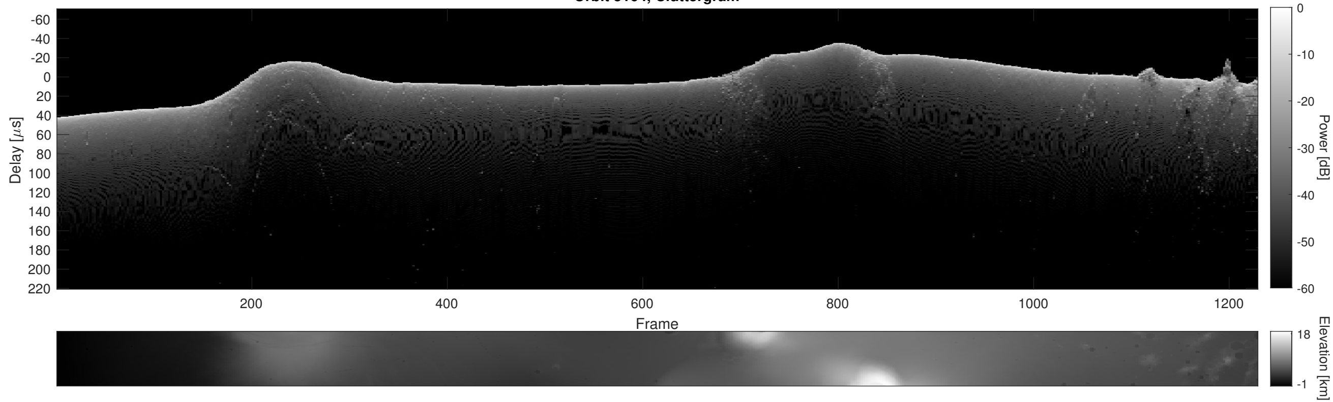
Orbit 5164, Cluttergram
