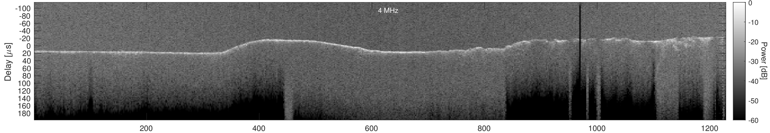
Orbit 5165, Cluttergram
