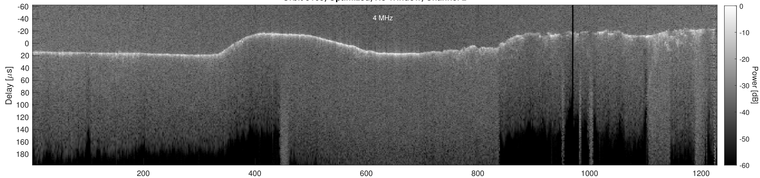
Orbit 5165, Cluttergram
