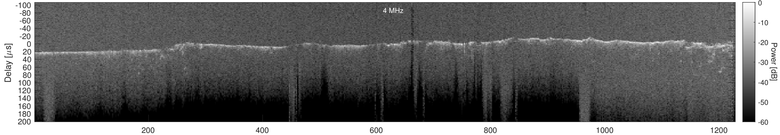
Orbit 5166, Cluttergram
