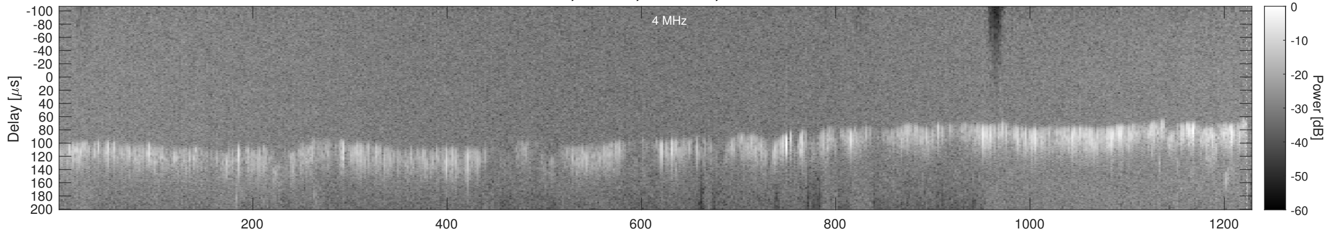
Orbit 5166, Window, Channel 2, Chapman
