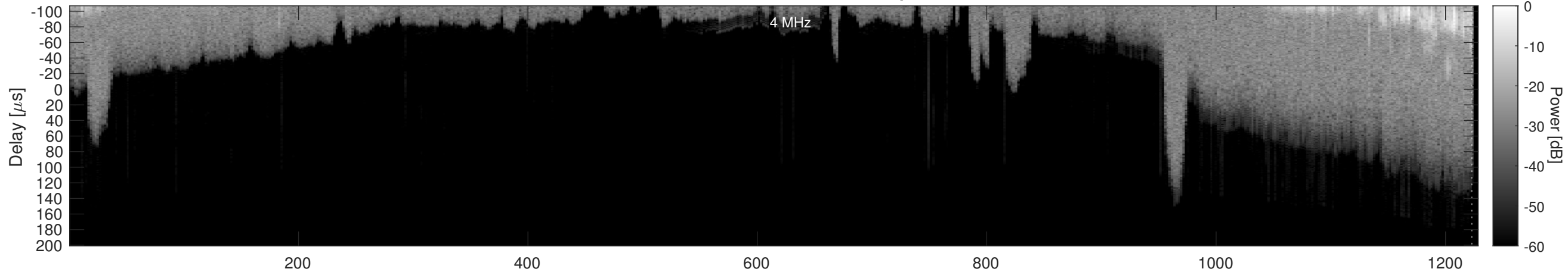
Orbit 5166, Window, Channel 2, Optimized
