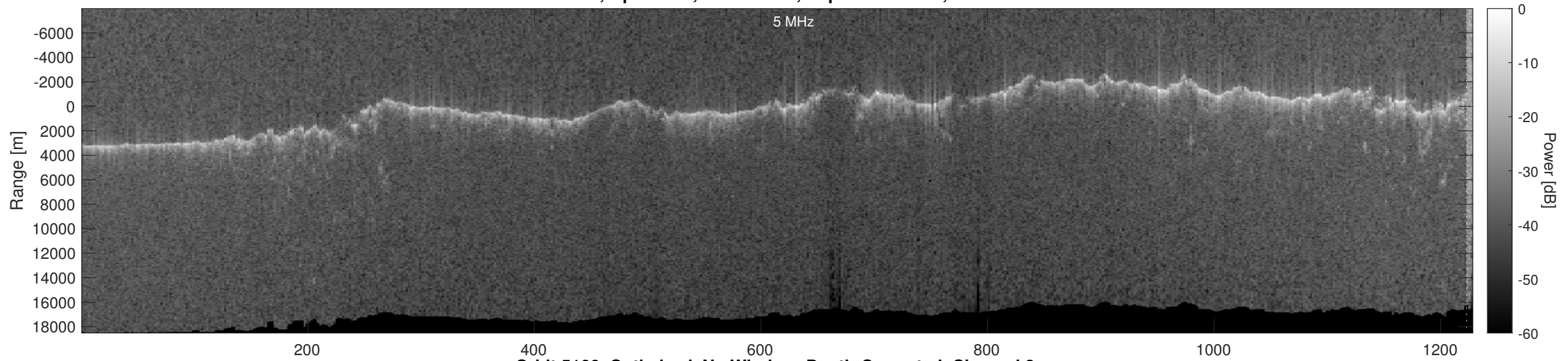
Orbit 5166, Optimized, No Window, Depth-Corrected, Channel 2
