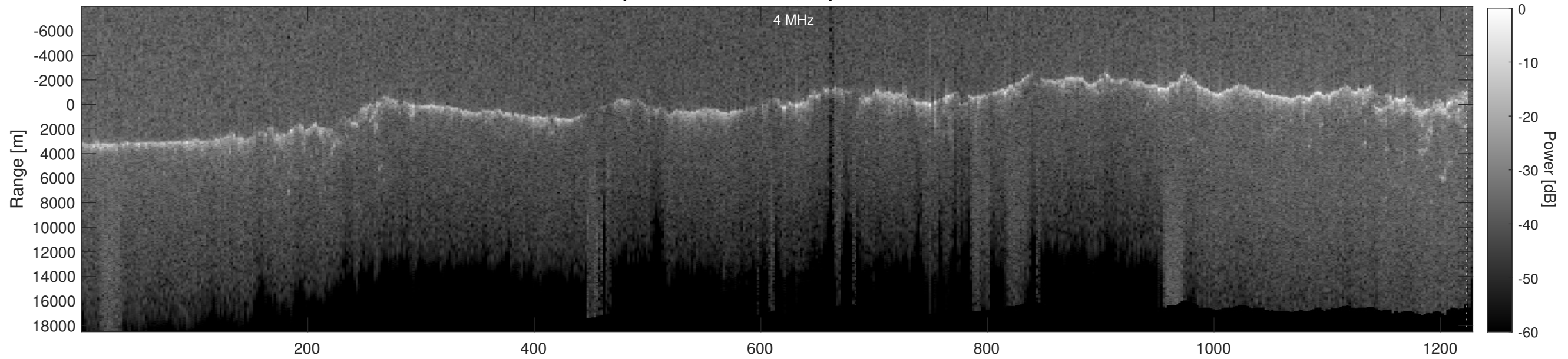
Orbit 5166, Depth-Corrected Cluttergram
