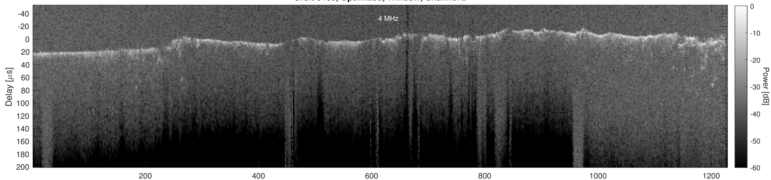
Orbit 5166, Cluttergram
