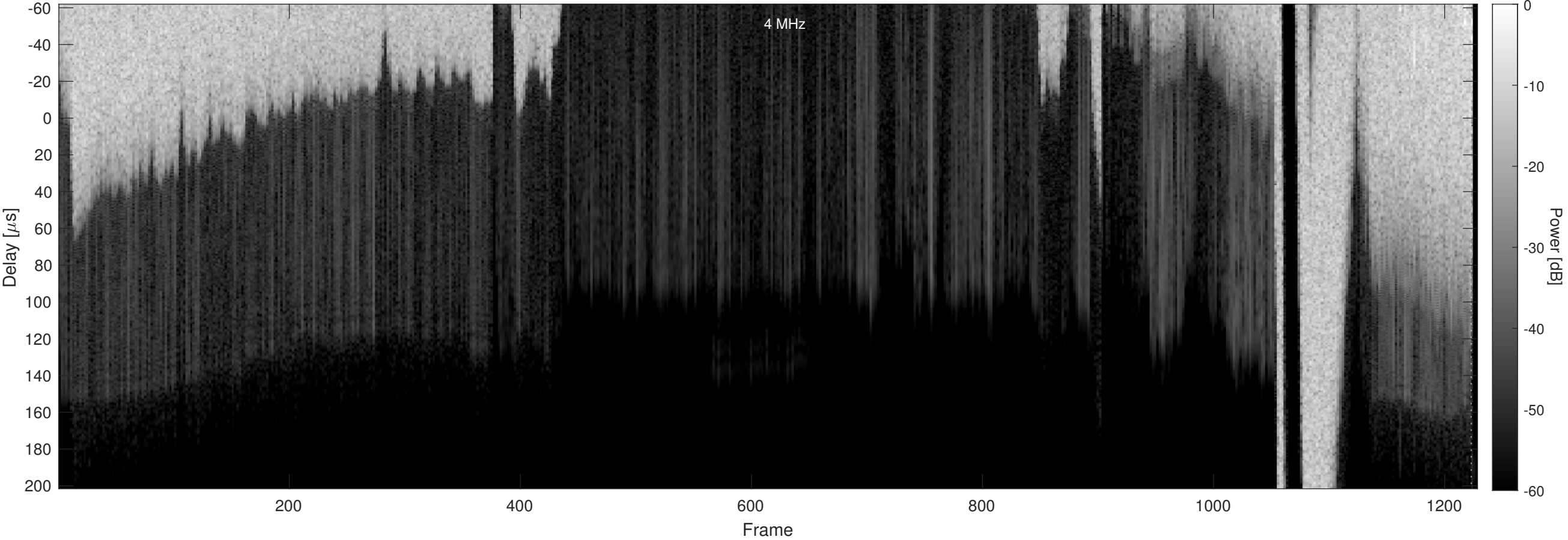
Orbit 5167, Chapman, Window, Channel 2
