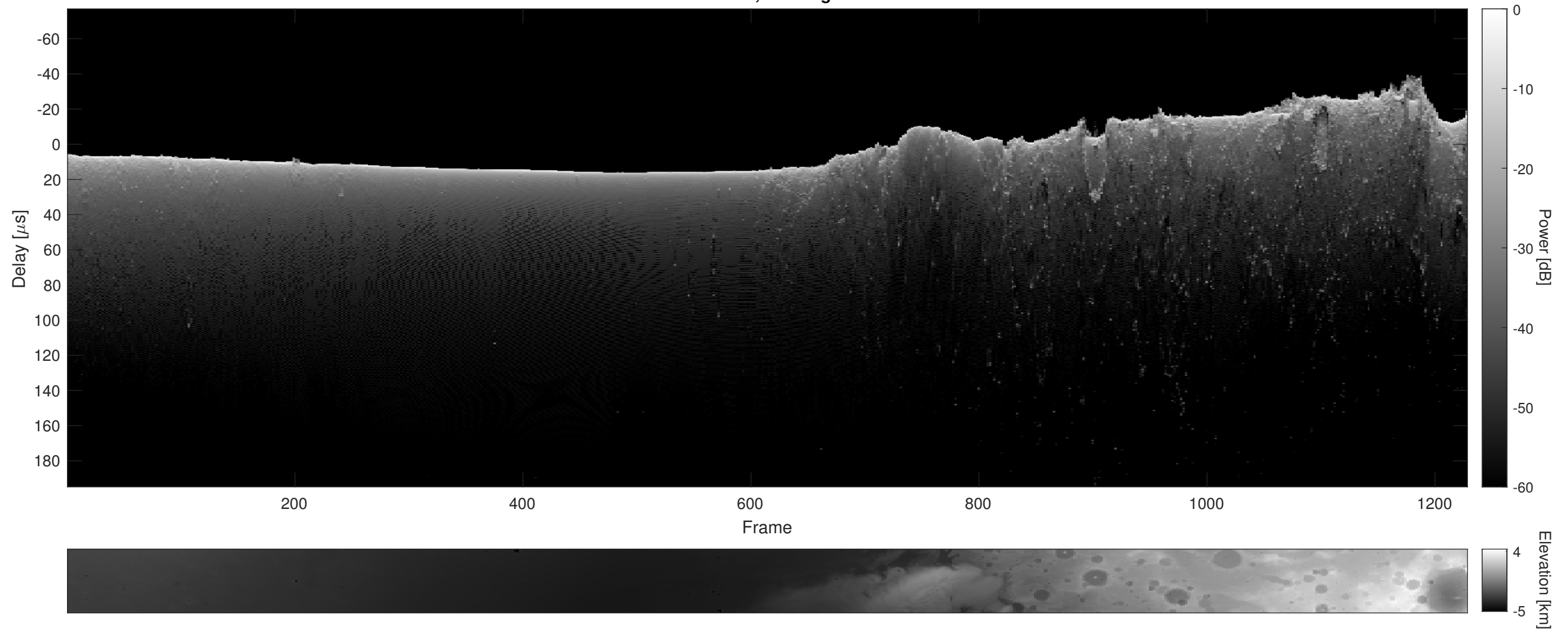
Orbit 5168, Cluttergram
