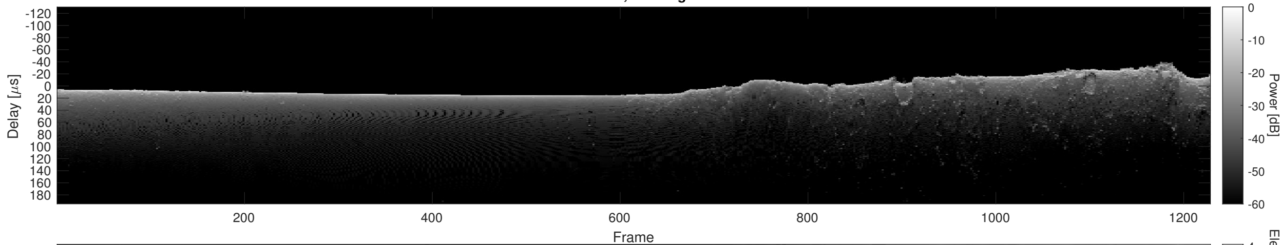
Orbit 5168, Cluttergram
