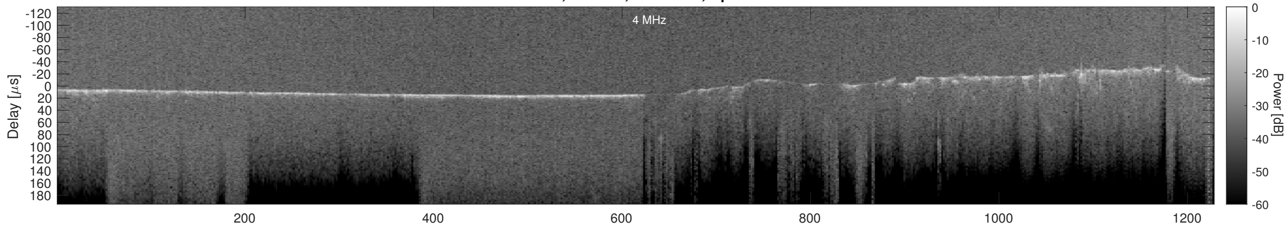
Orbit 5168, Cluttergram
