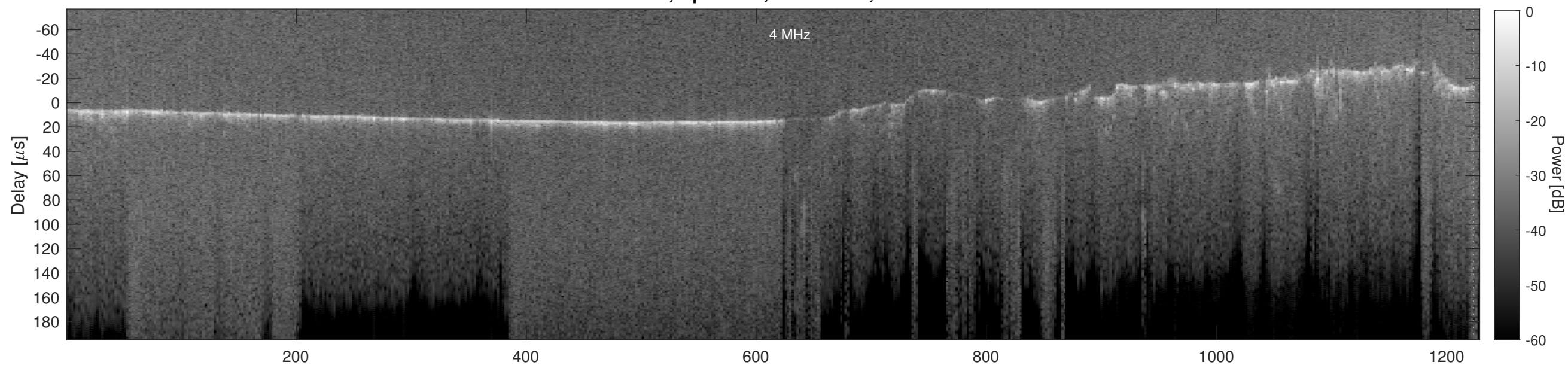
Orbit 5168, Cluttergram
