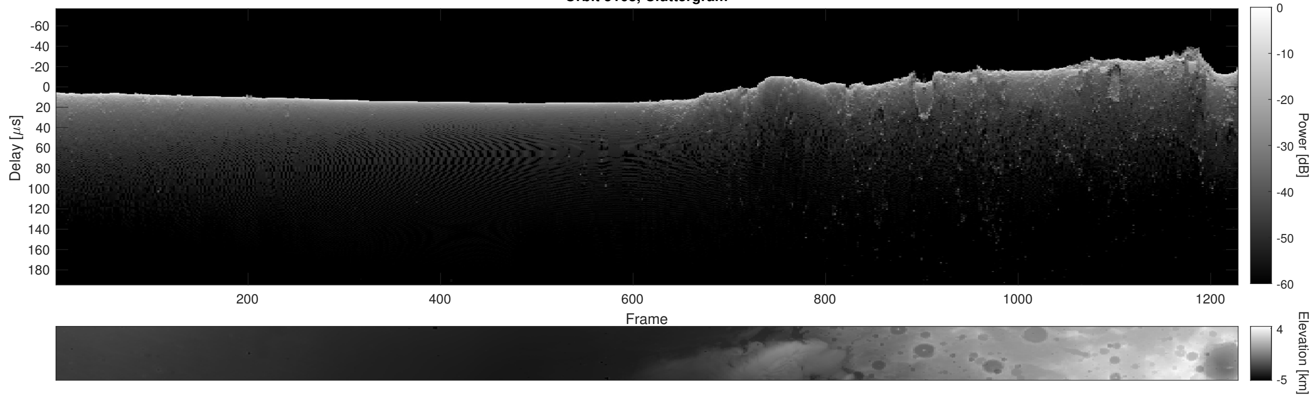
Orbit 5168, Cluttergram
