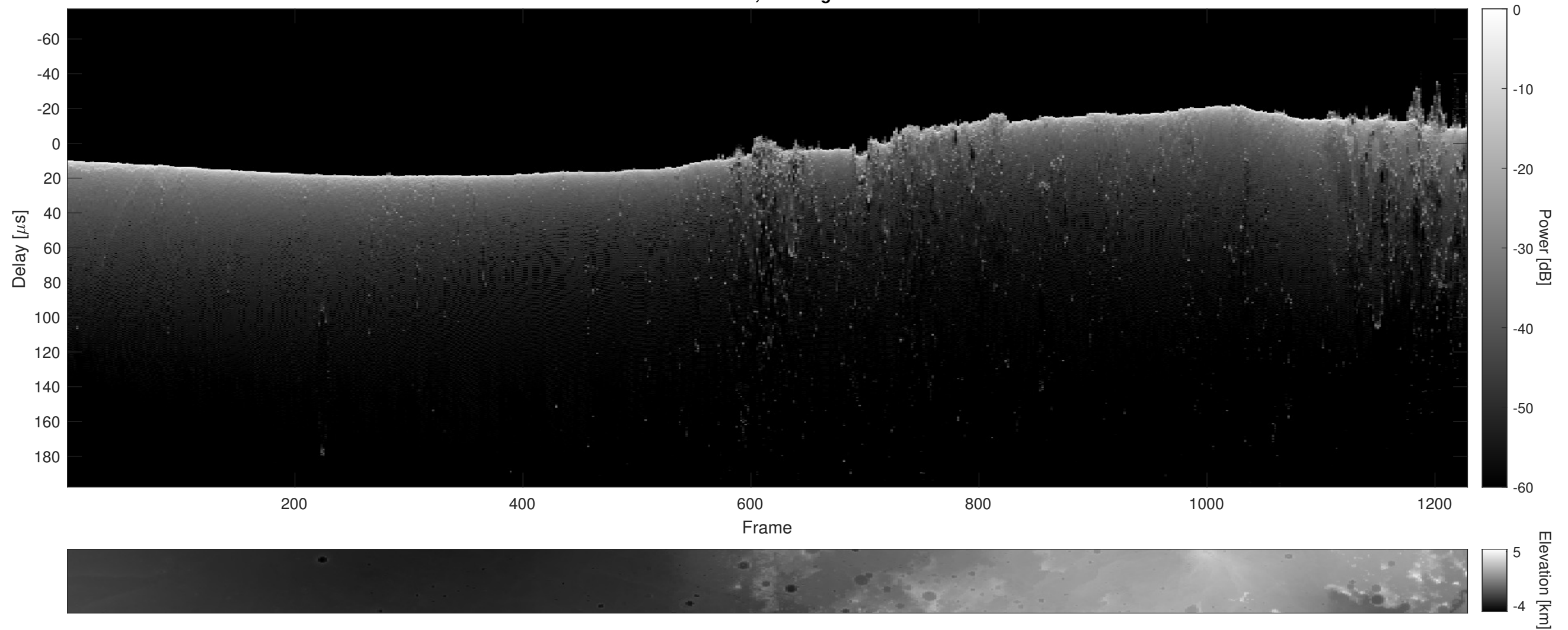
Orbit 5169, Cluttergram
