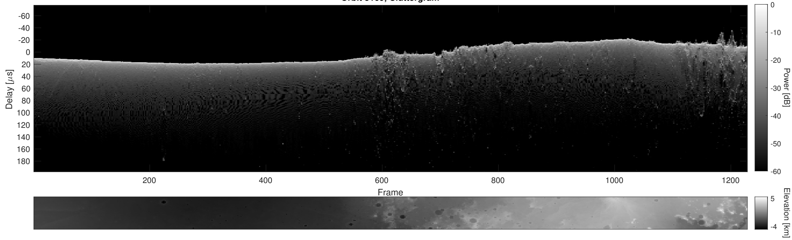
Orbit 5169, Cluttergram
