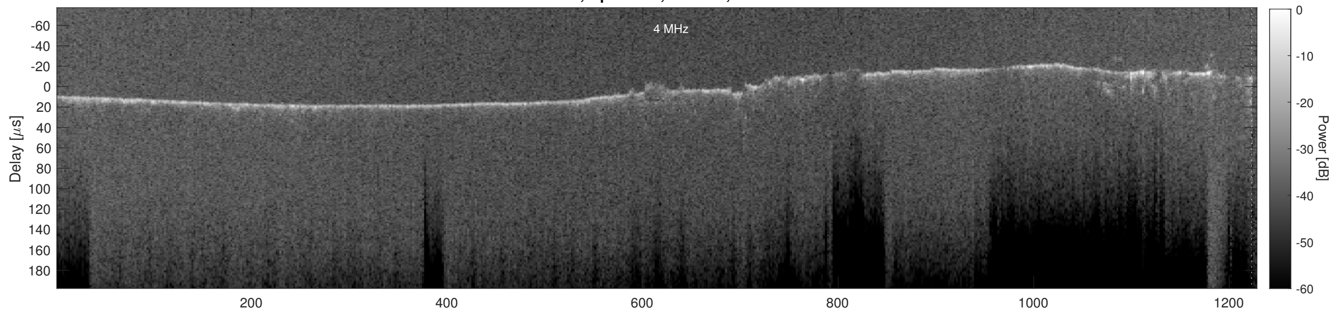
Orbit 5169, Cluttergram
