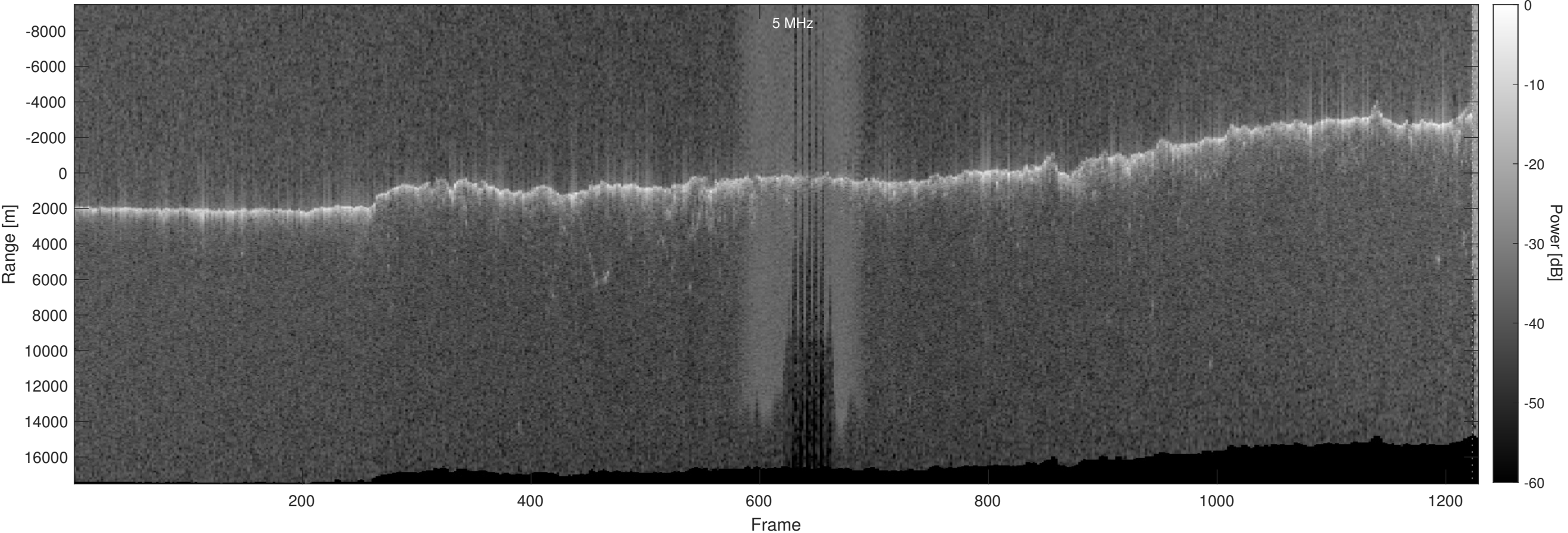
Orbit 5170, Optimized, No Window, Depth-Corrected, Channel 2
