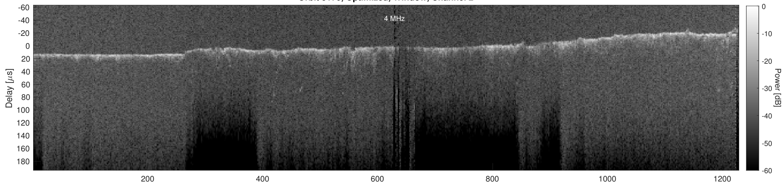
Orbit 5170, Cluttergram
