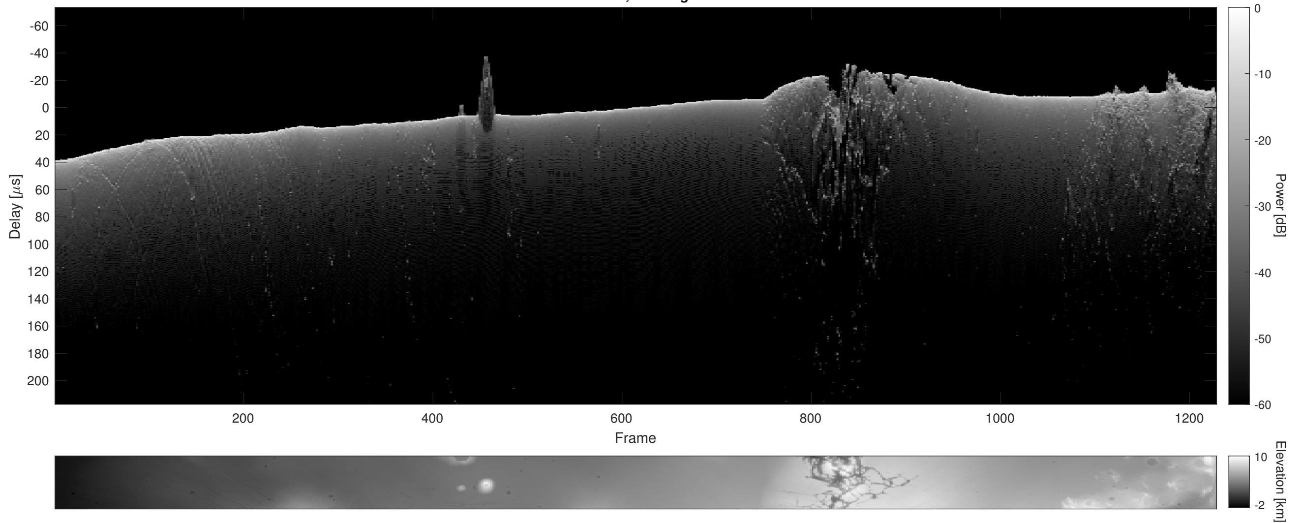
Orbit 5171, Cluttergram
