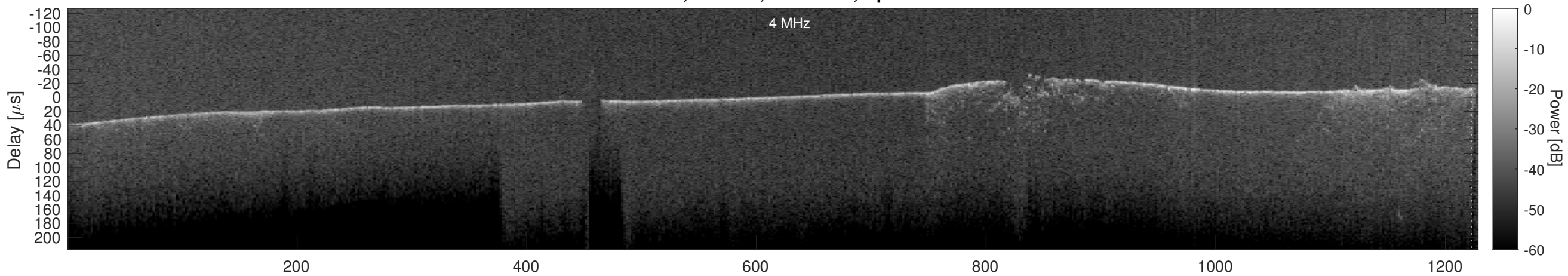
Orbit 5171, Cluttergram
