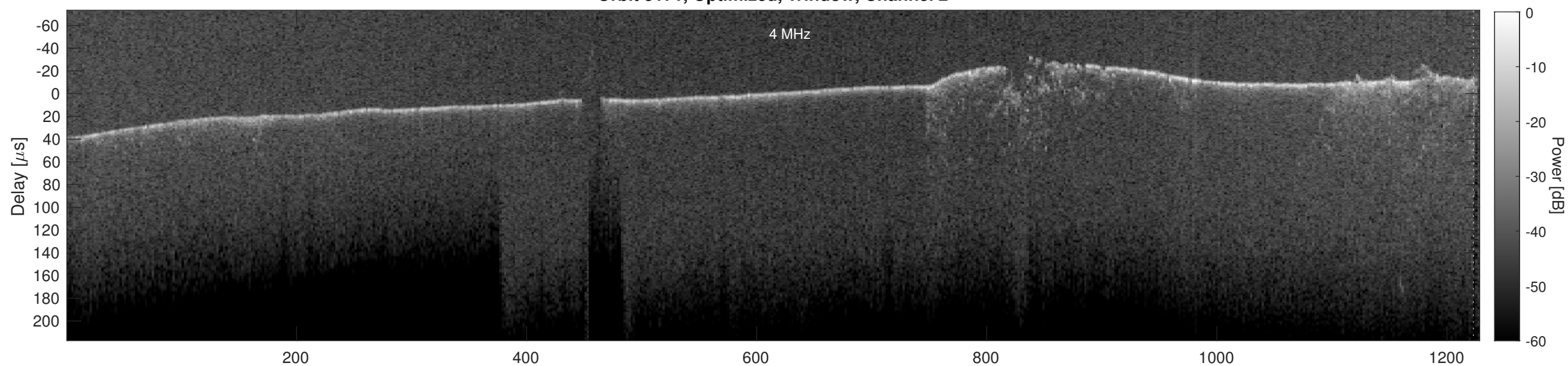
Orbit 5171, Cluttergram
