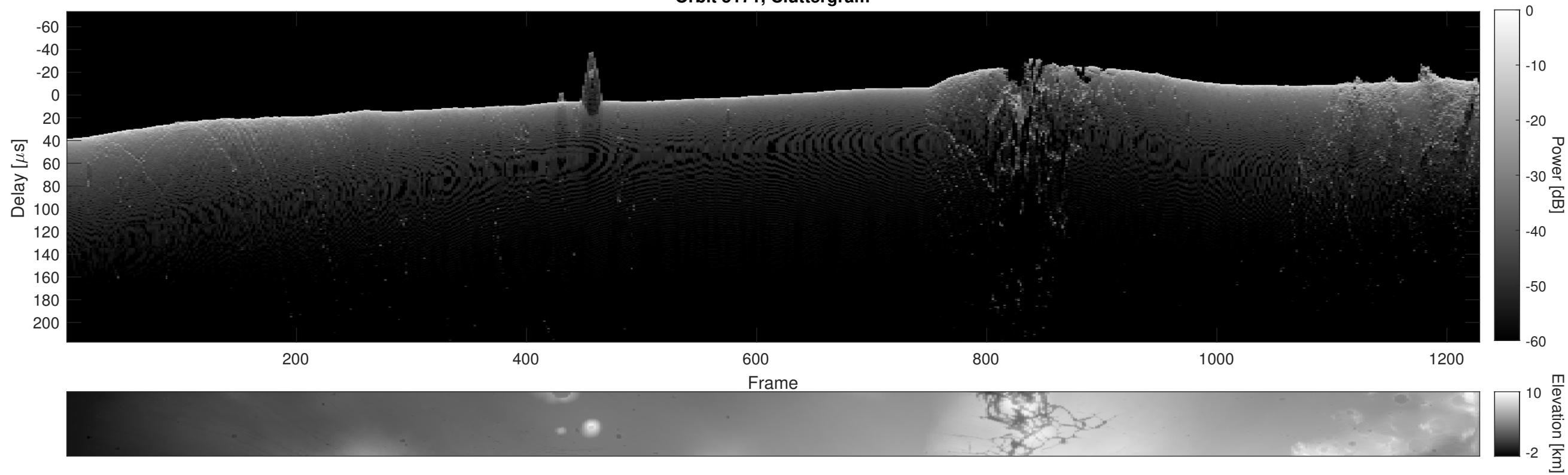
Orbit 5171, Cluttergram
