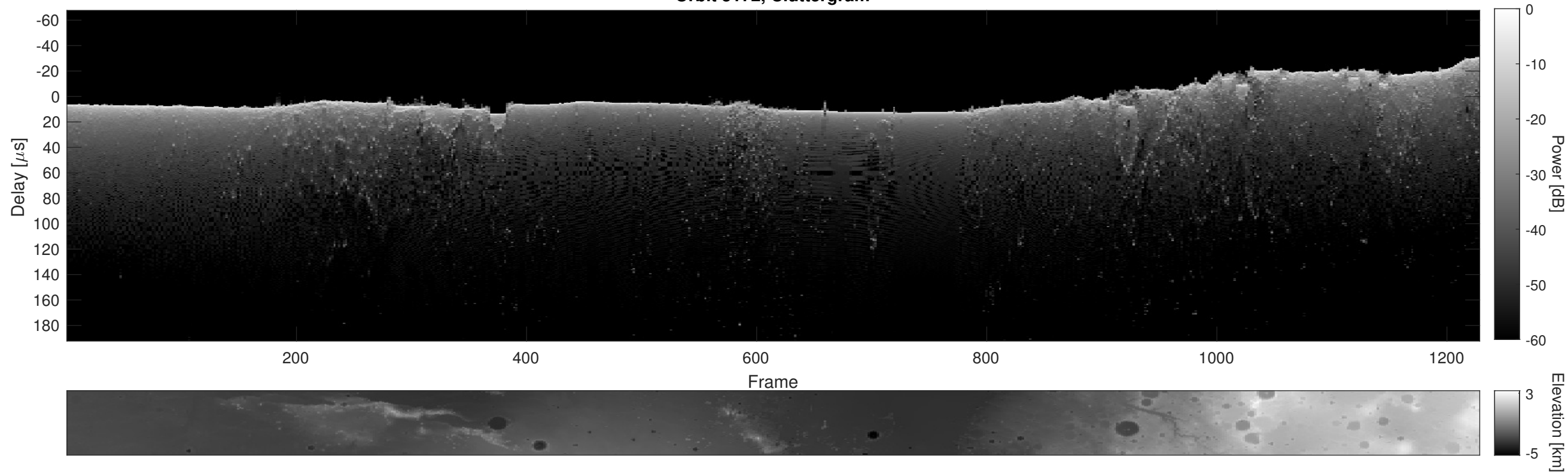
Orbit 5172, Cluttergram
