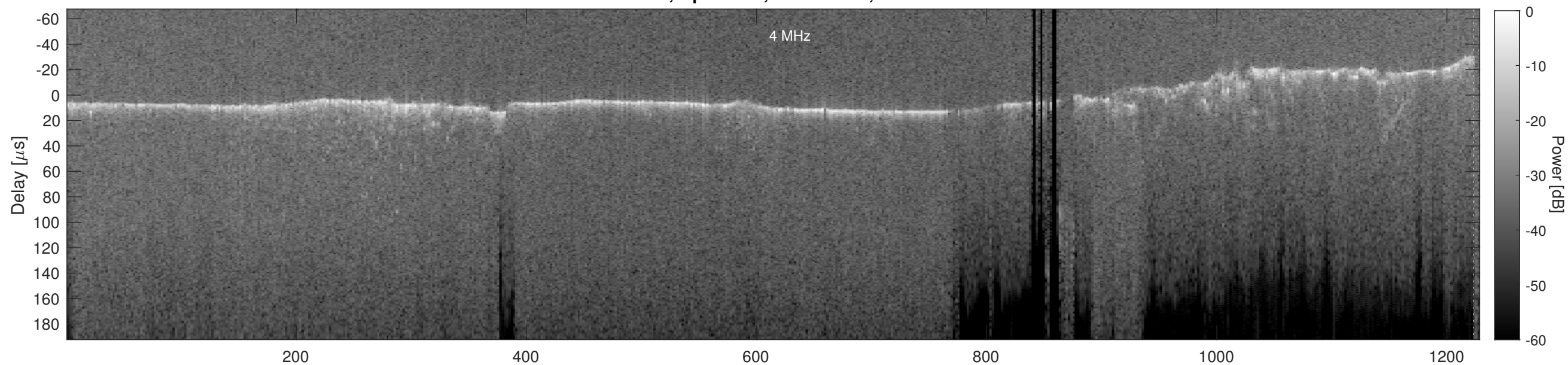
Orbit 5172, Cluttergram
