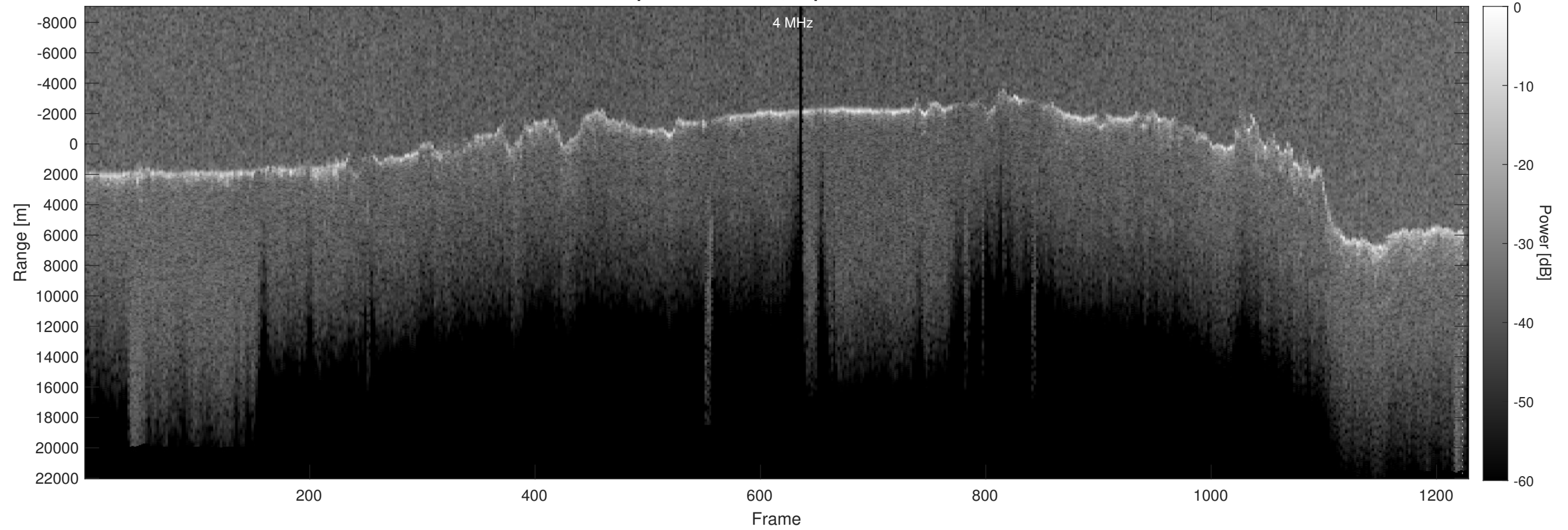
Orbit 5173, Optimized, Window, Depth-Corrected, Channel 2
