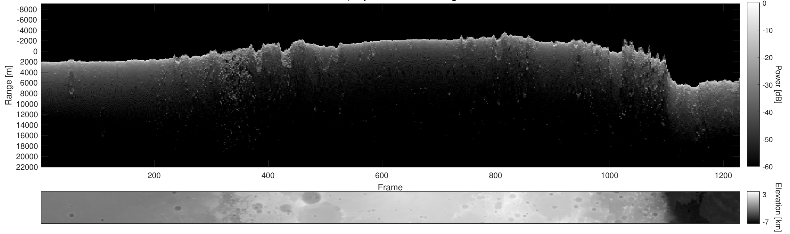
Orbit 5173, Depth-Corrected Cluttergram
