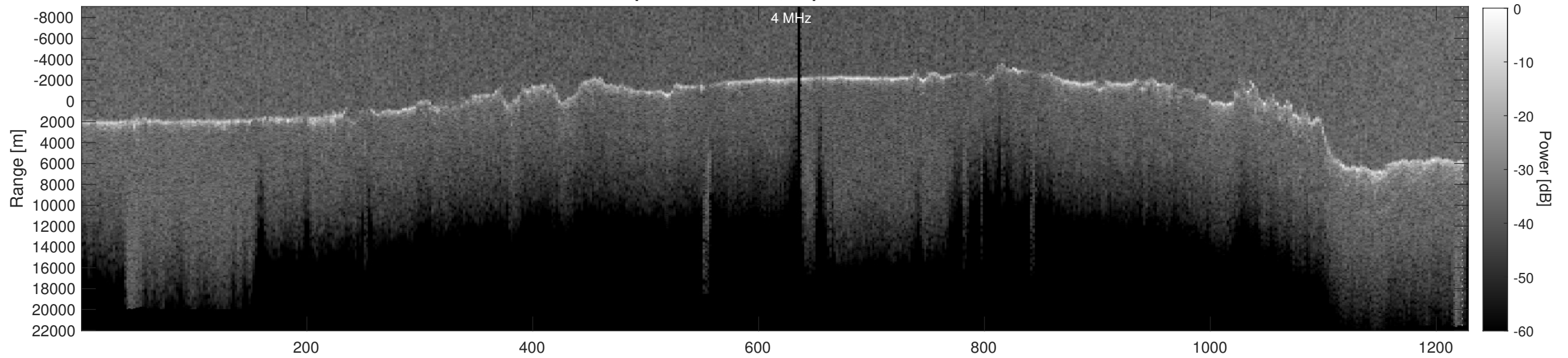
Orbit 5173, Depth-Corrected Cluttergram
