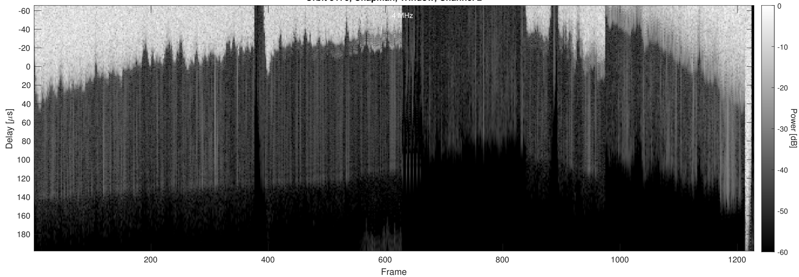
Orbit 5176, Chapman, Window, Channel 2
