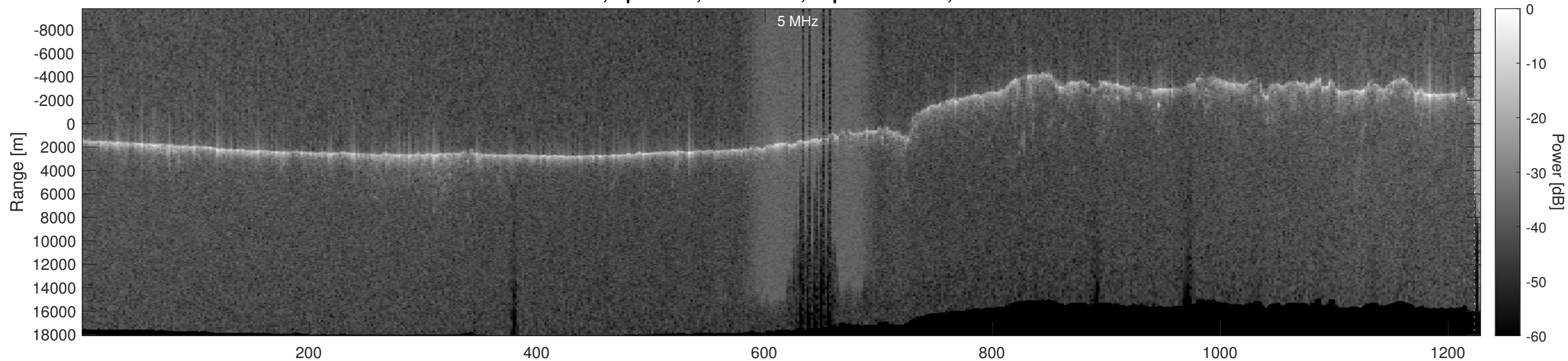
Orbit 5176, Optimized, No Window, Depth-Corrected, Channel 2
