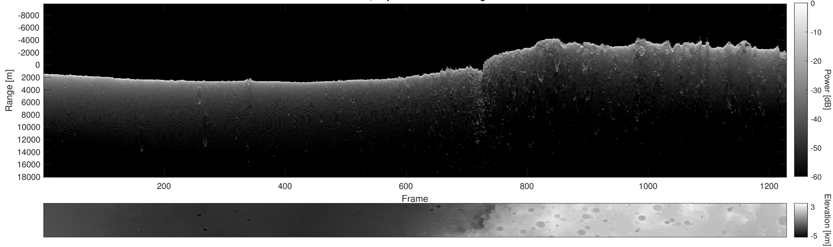
Orbit 5176, Depth-Corrected Cluttergram
