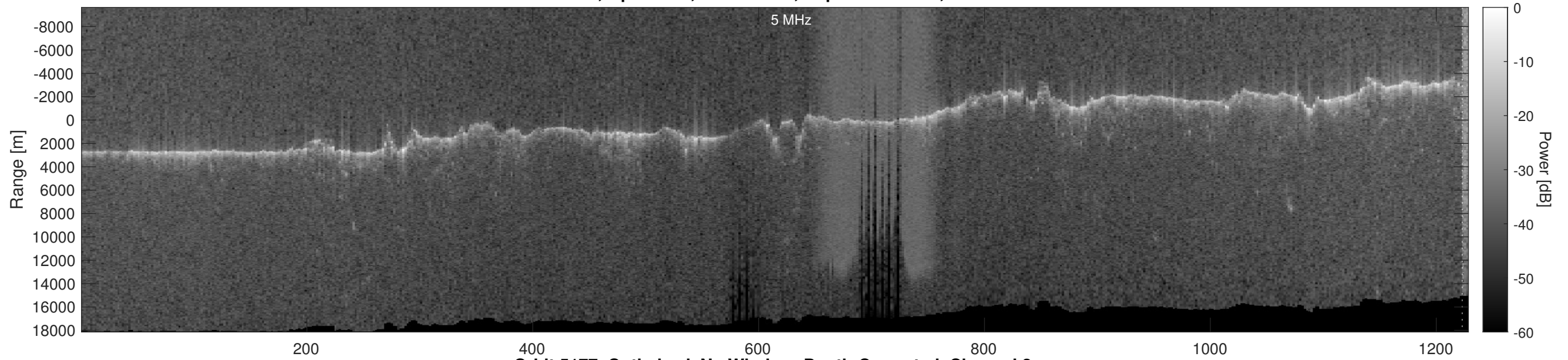
Orbit 5177, Optimized, No Window, Depth-Corrected, Channel 2
