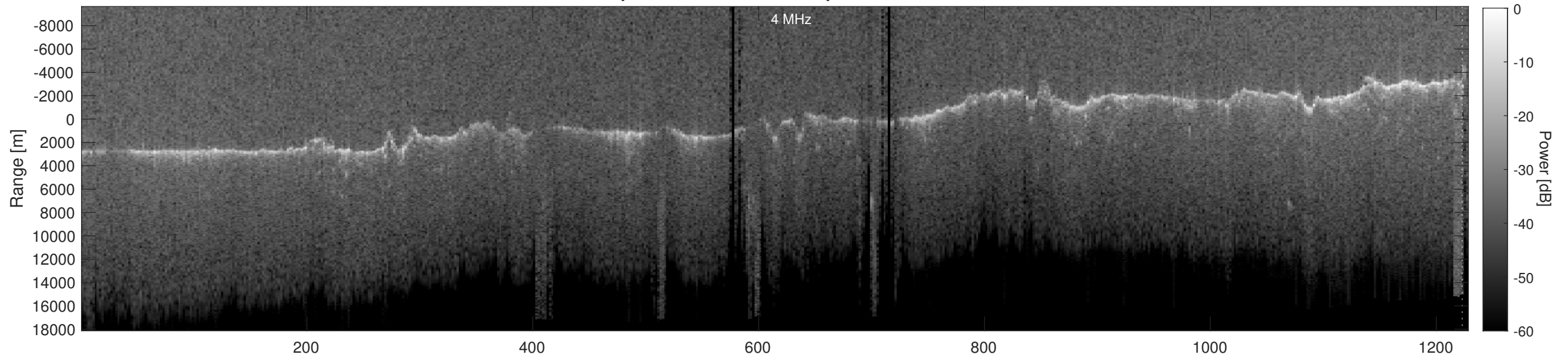
Orbit 5177, Depth-Corrected Cluttergram
