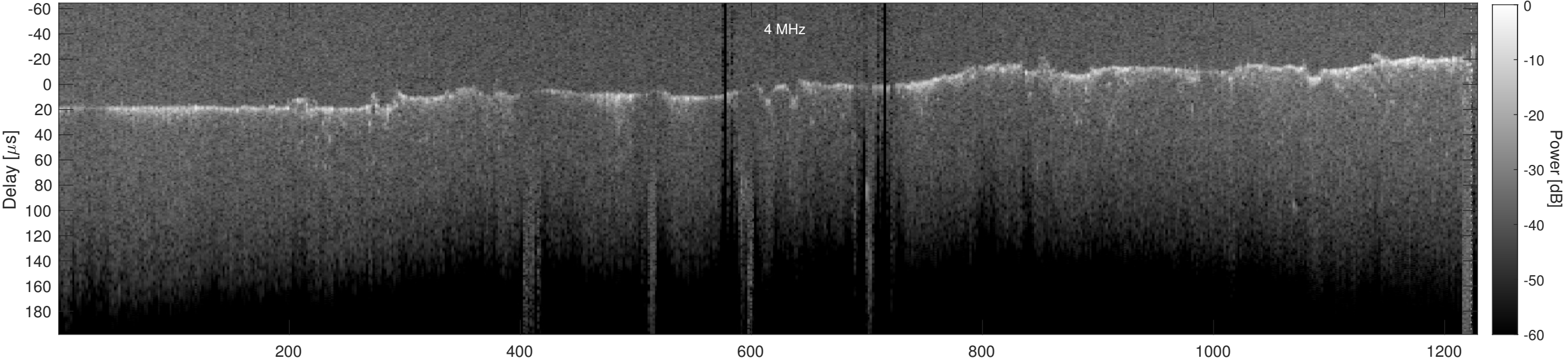
Orbit 5177, Cluttergram
