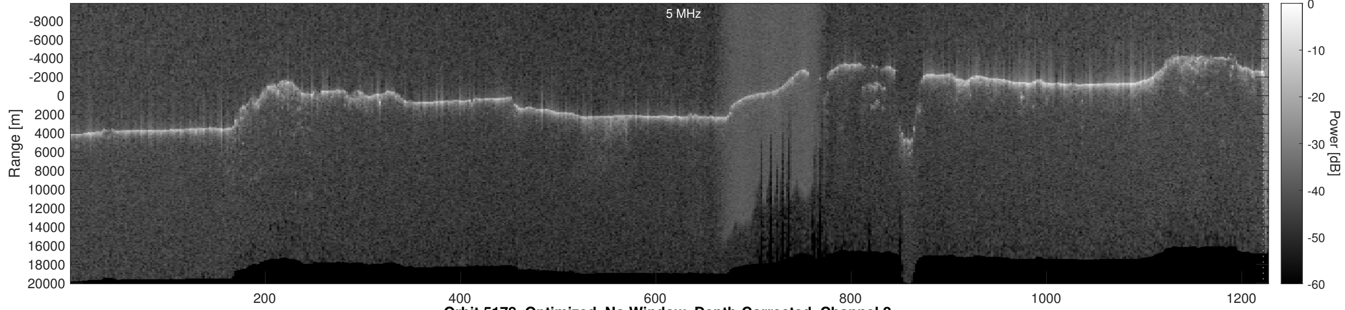
Orbit 5178, Optimized, No Window, Depth-Corrected, Channel 2
