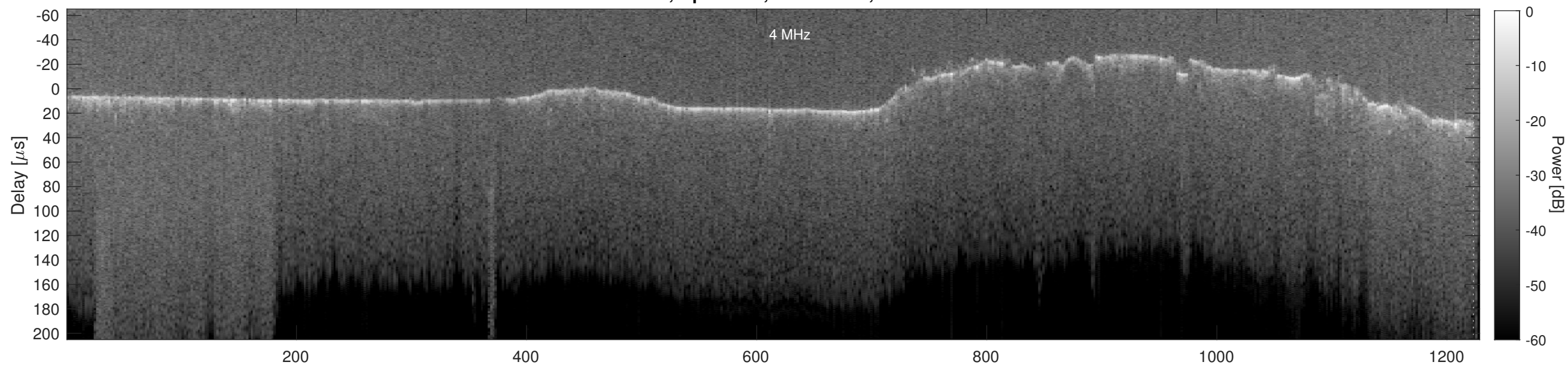
Orbit 5180, Cluttergram
