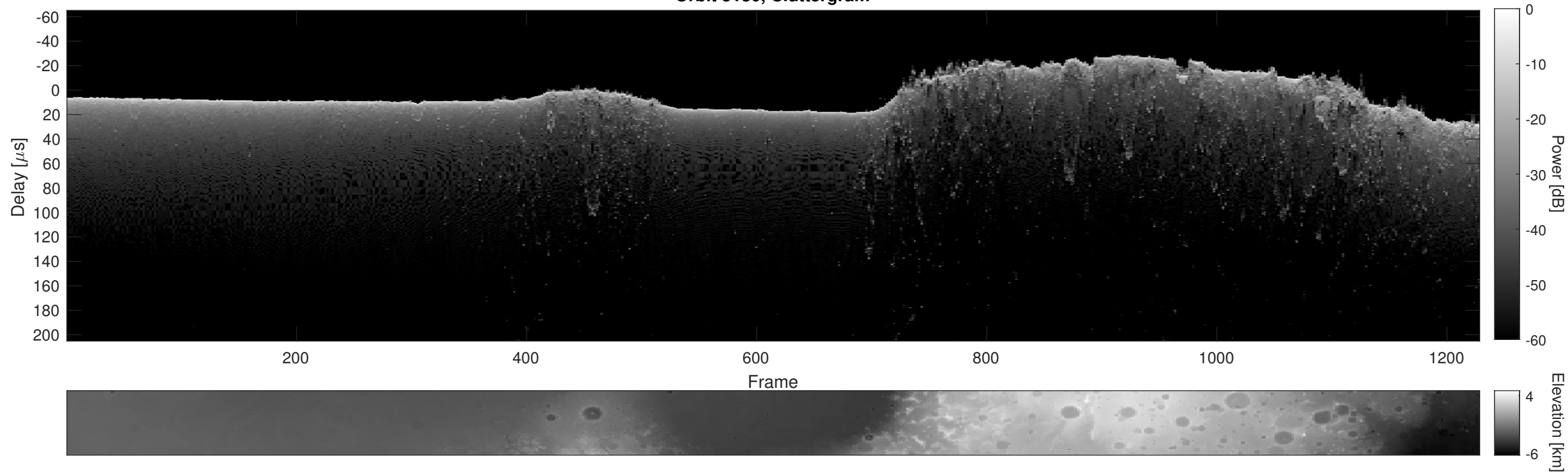
Orbit 5180, Cluttergram
