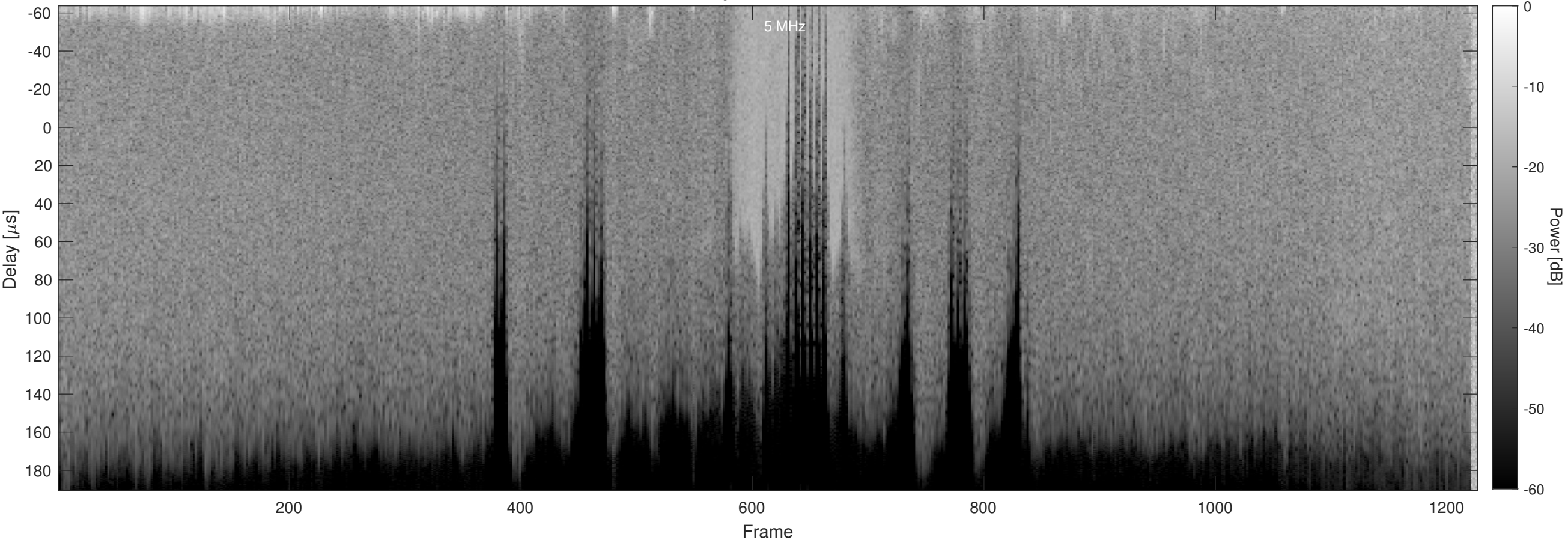
Orbit 5181, Chapman, Window, Channel 2
