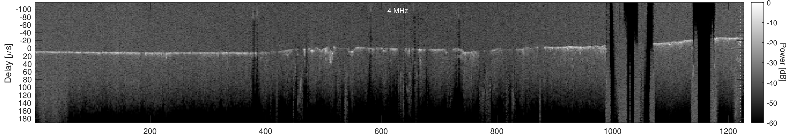
Orbit 5181, Cluttergram
