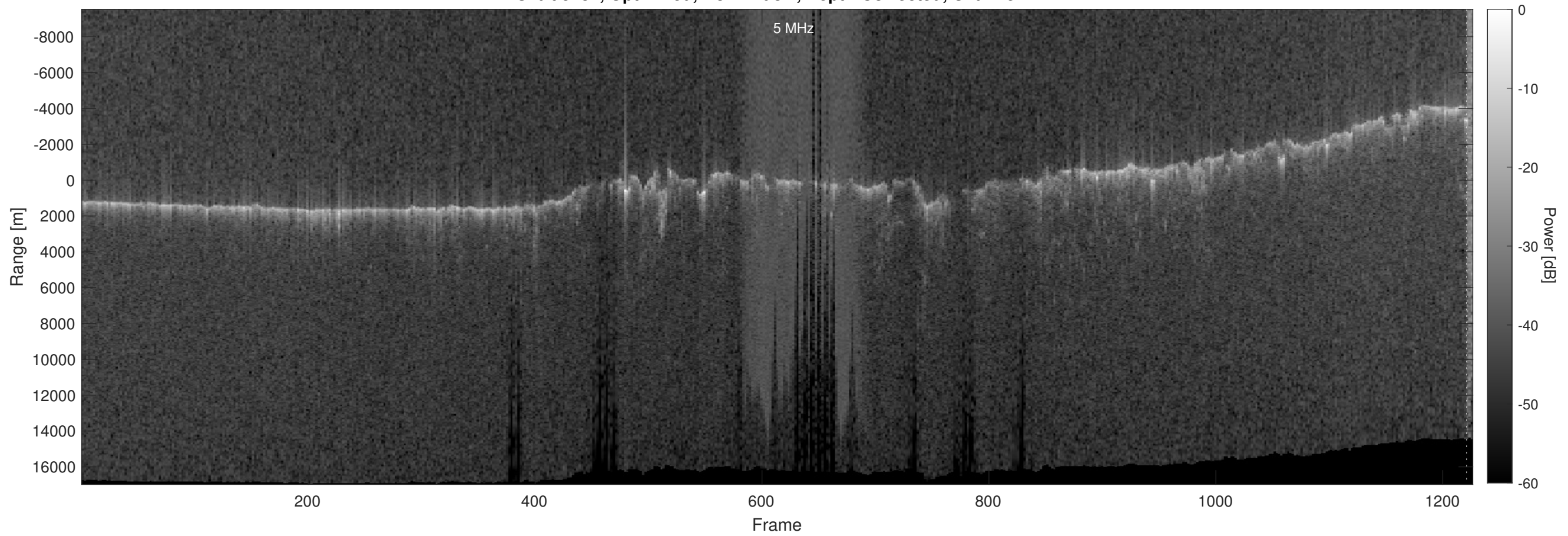
Orbit 5181, Optimized, No Window, Depth-Corrected, Channel 2
