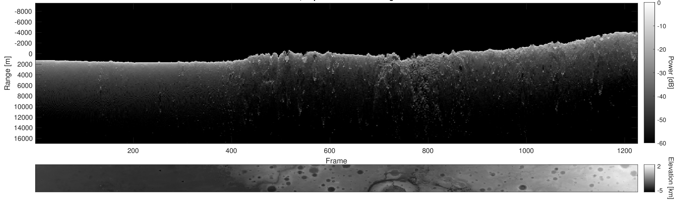
Orbit 5181, Depth-Corrected Cluttergram
