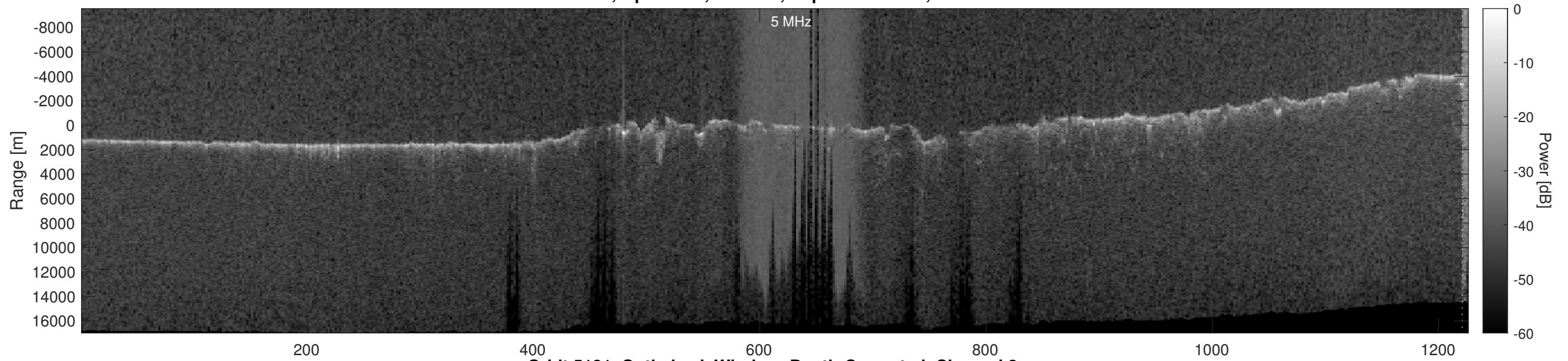
Orbit 5181, Optimized, Window, Depth-Corrected, Channel 2
