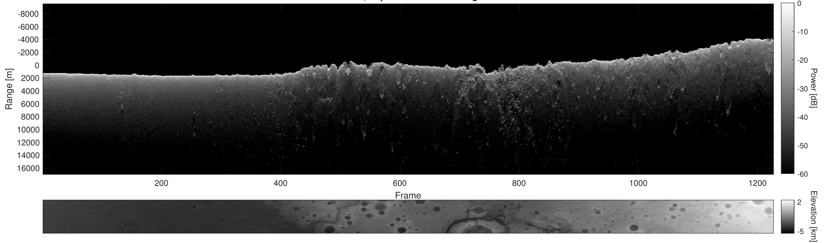
Orbit 5181, Depth-Corrected Cluttergram
