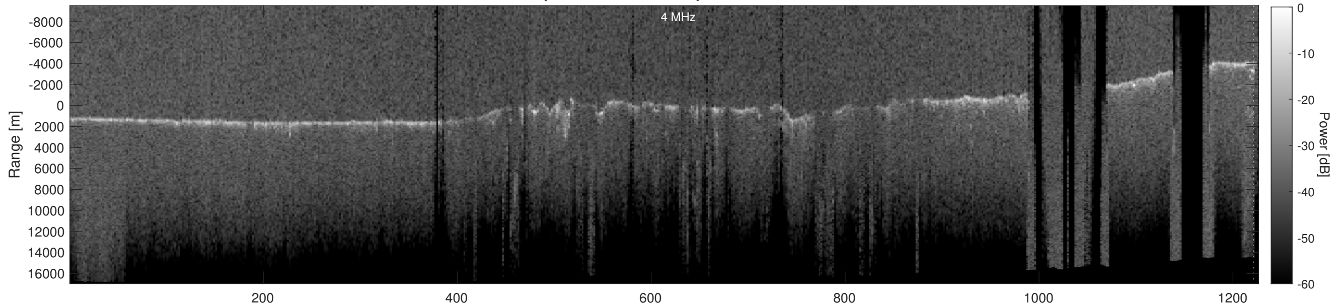
Orbit 5181, Depth-Corrected Cluttergram
