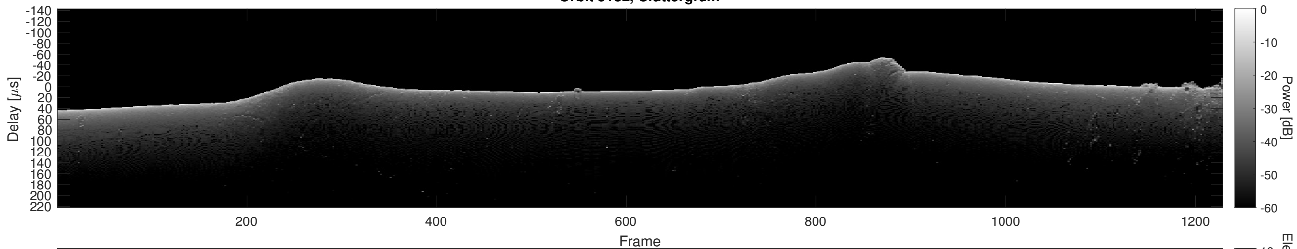
Orbit 5182, Cluttergram
