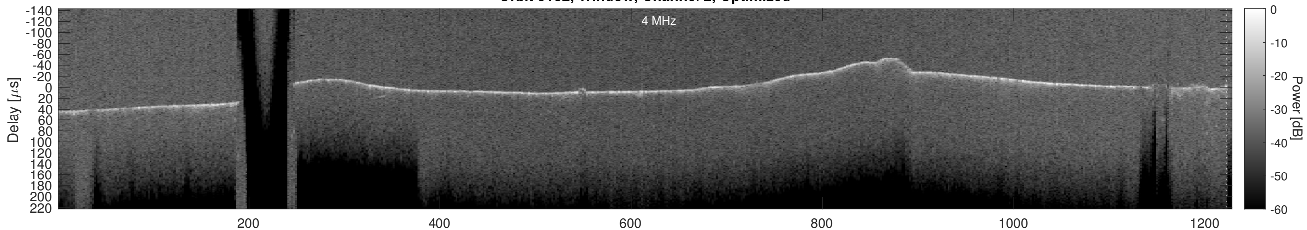
Orbit 5182, Cluttergram
