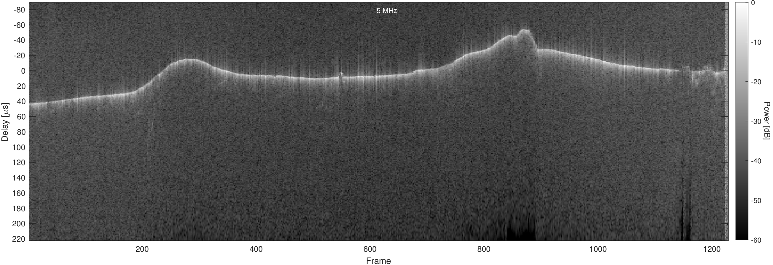
Orbit 5182, Optimized, No Window, Channel 2
