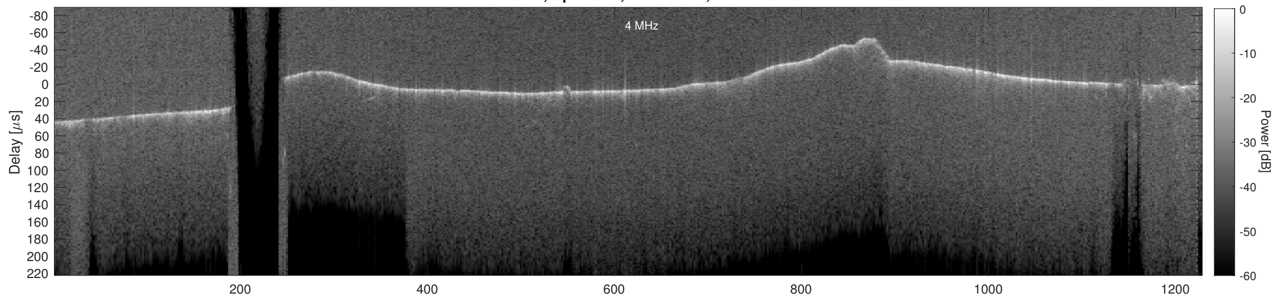
Orbit 5182, Cluttergram
