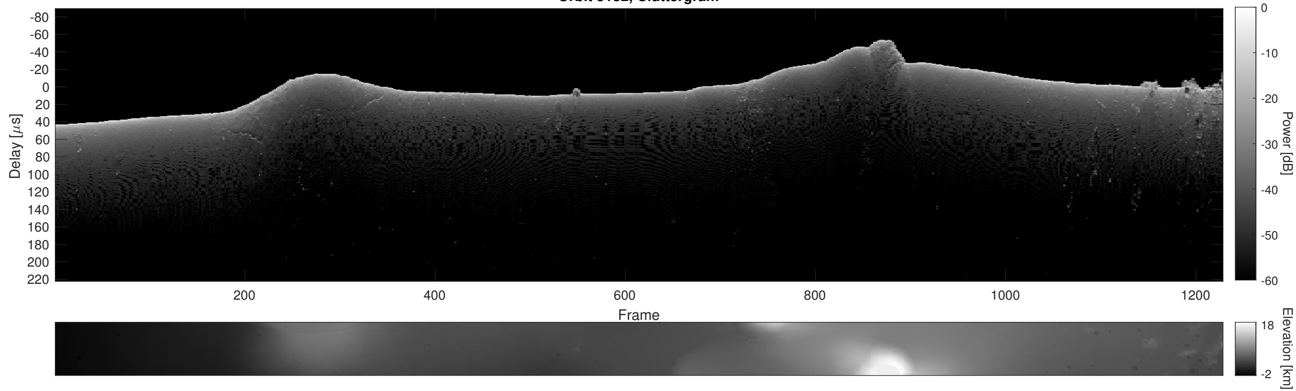
Orbit 5182, Cluttergram
