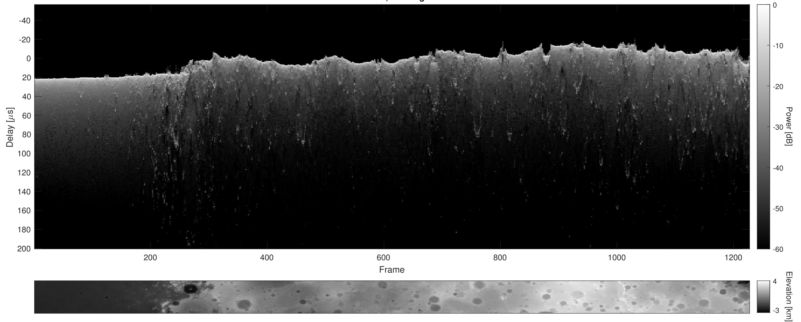
Orbit 5184, Cluttergram
