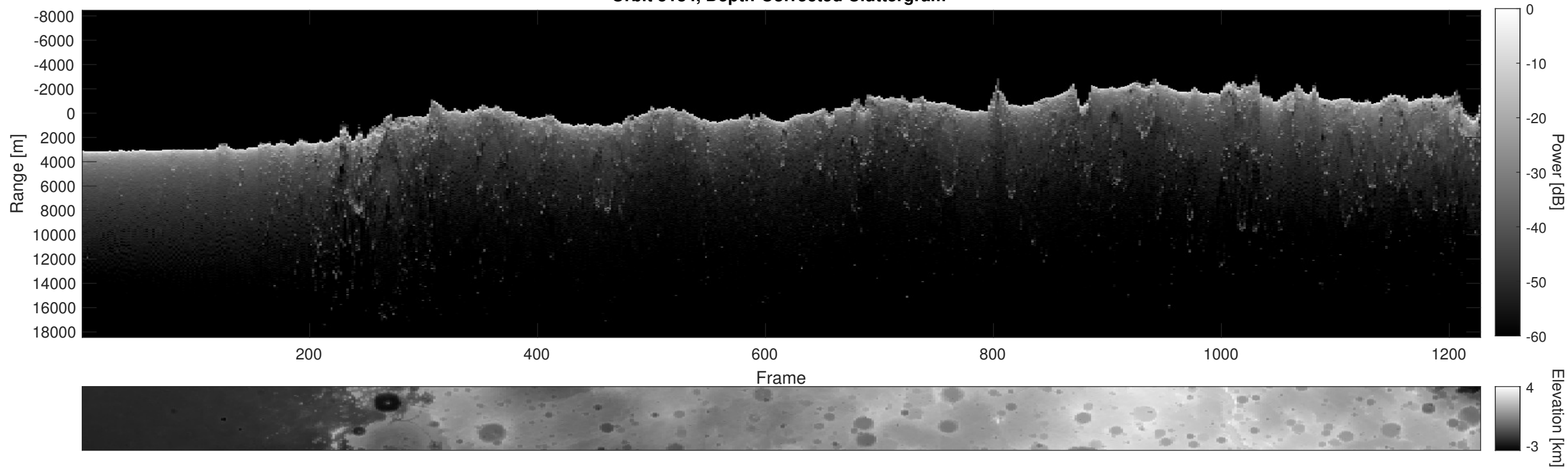
Orbit 5184, Depth-Corrected Cluttergram
