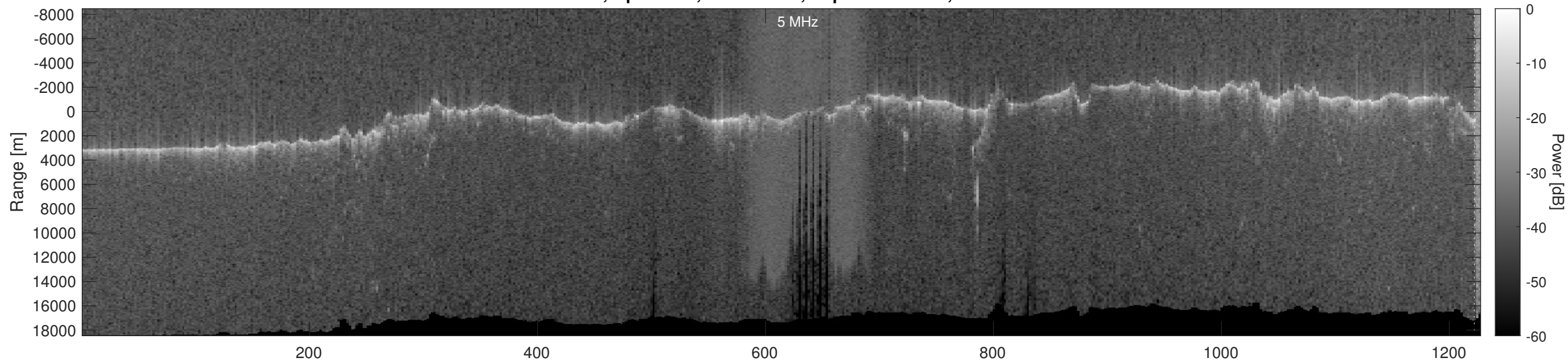
Orbit 5184, Optimized, No Window, Depth-Corrected, Channel 2
