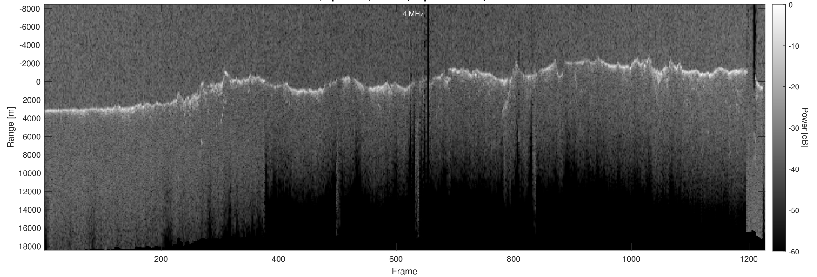
Orbit 5184, Optimized, Window, Depth-Corrected, Channel 2
