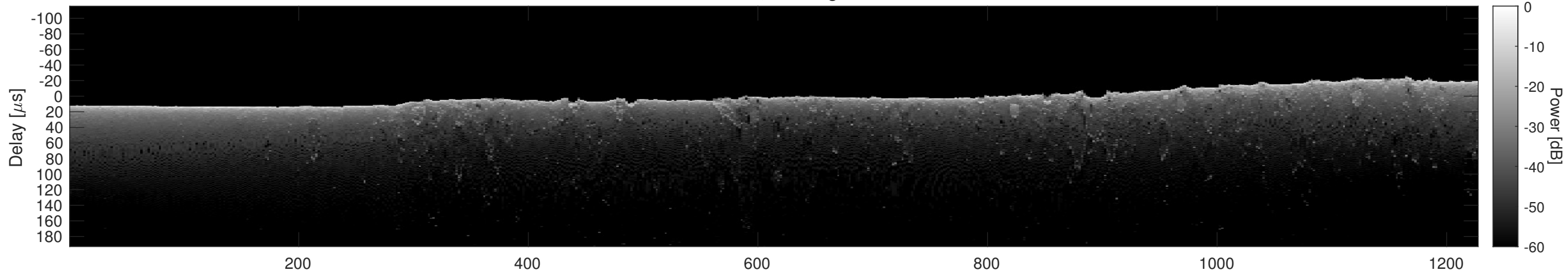
Orbit 5188, Cluttergram
