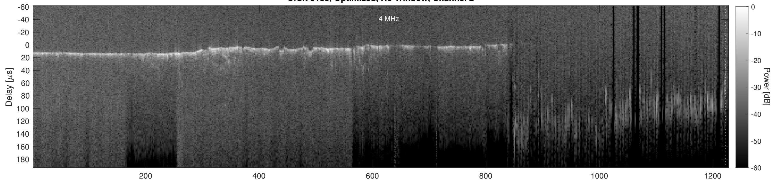
Orbit 5188, Cluttergram
