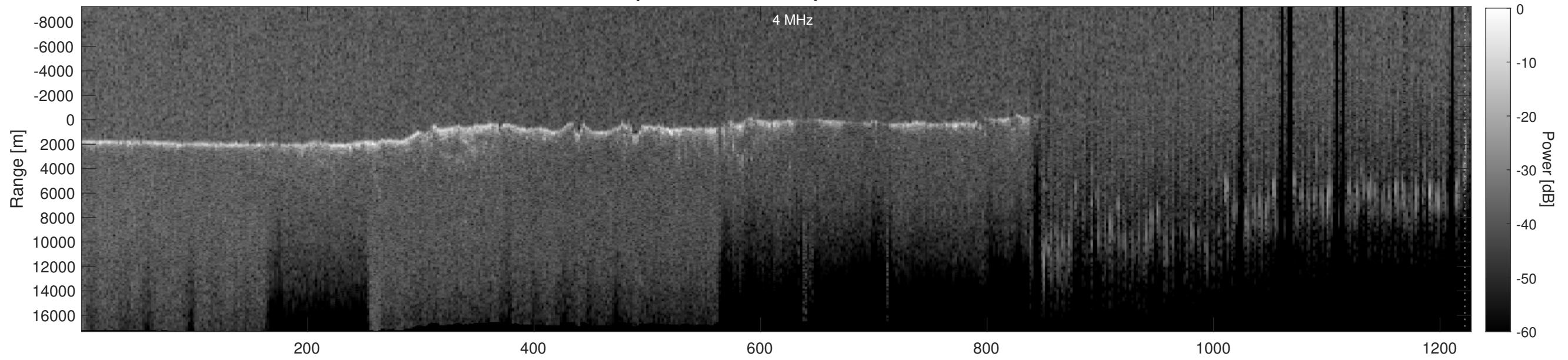
Orbit 5188, Depth-Corrected Cluttergram
