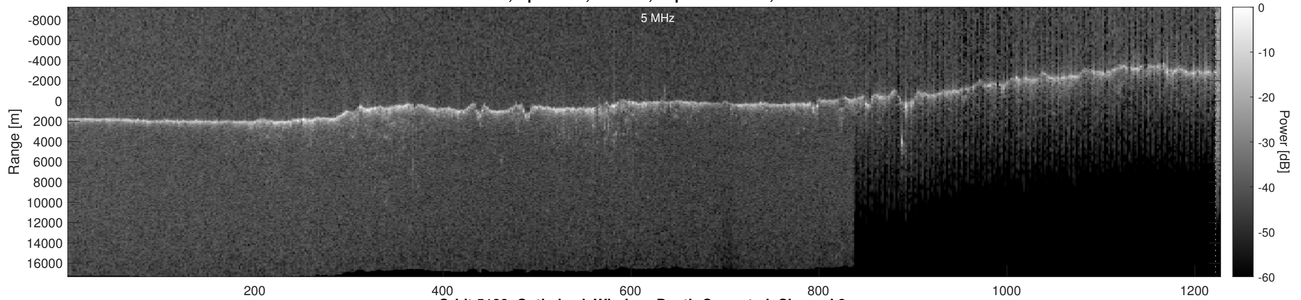
Orbit 5188, Optimized, Window, Depth-Corrected, Channel 2
