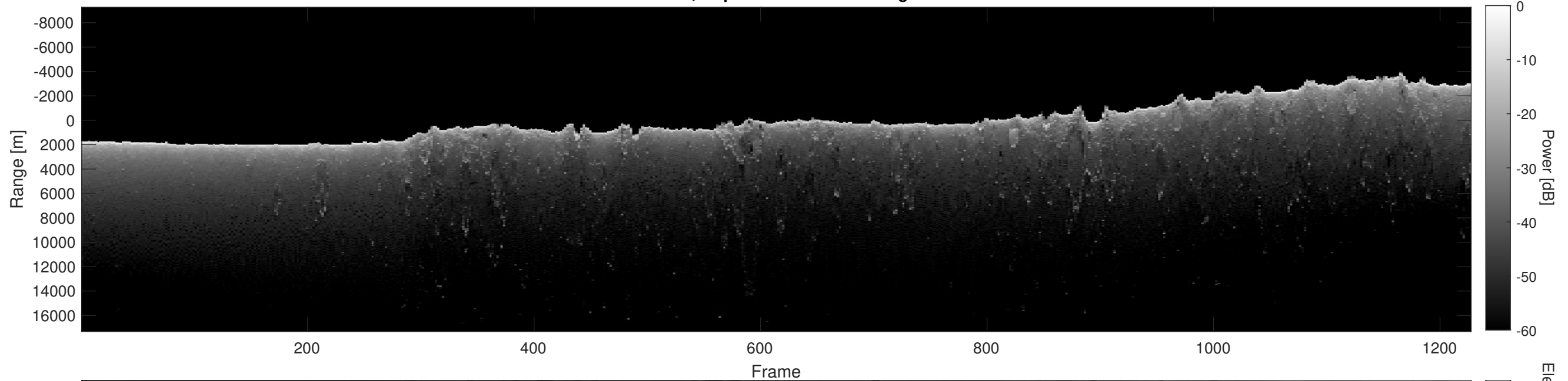
Orbit 5188, Depth-Corrected Cluttergram
